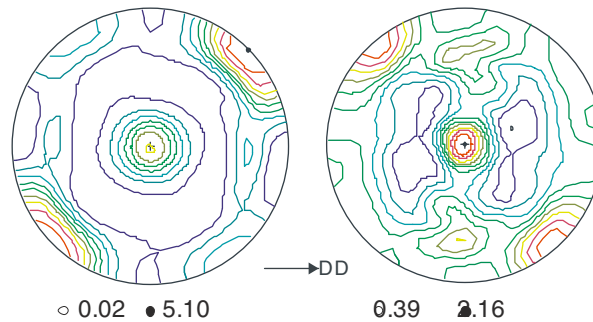
Fig. 30. (0002) (left) and (10 \bar{1} 0) (right) pole figures after simple shear loading in D.D. at room temperature ( 25^\circ\text{C} ) and strain rate of 10^0\text{ s}^{-1} .
