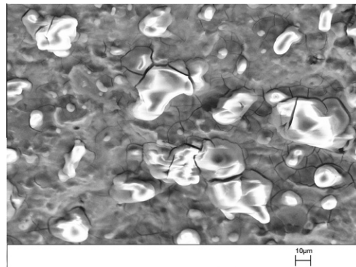
Fig. 31. Fracture surface of the tensile specimen deformed in RD at the strain rate of 10^{-2}\text{ s}^{-1} at room temperature ( 25^\circ\text{C} ).
