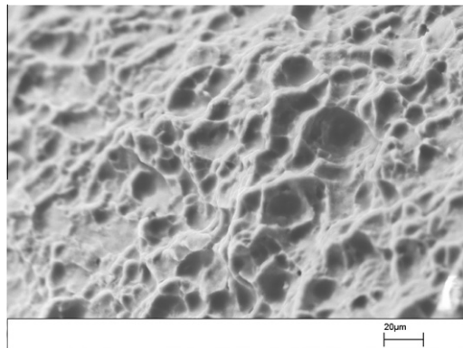
Fig. 32. Fracture surface of the tensile specimen deformed in RD at the strain rate of 10^{-2} \text{ s}^{-1} at 150^\circ\text{C} .
