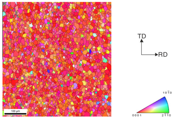
Fig. 15. Inverse pole figure (IPF) EBSD map of as-received sheet.
