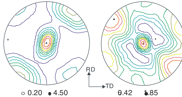
Fig. 29. (0002) (left) and (10 \bar{1} 0) (right) pole figures after simple shear loading in TD at room temperature ( 25^\circ\text{C} ) and strain rate of 10^0\text{ s}^{-1} .
