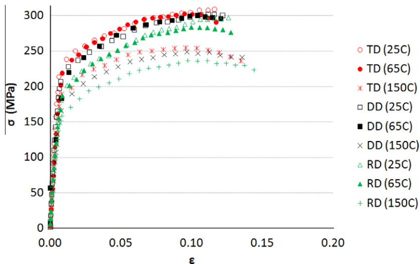
Fig. 2. Tension (true) responses at a strain rate of 10 0 s -1 at different temperatures and directions.
