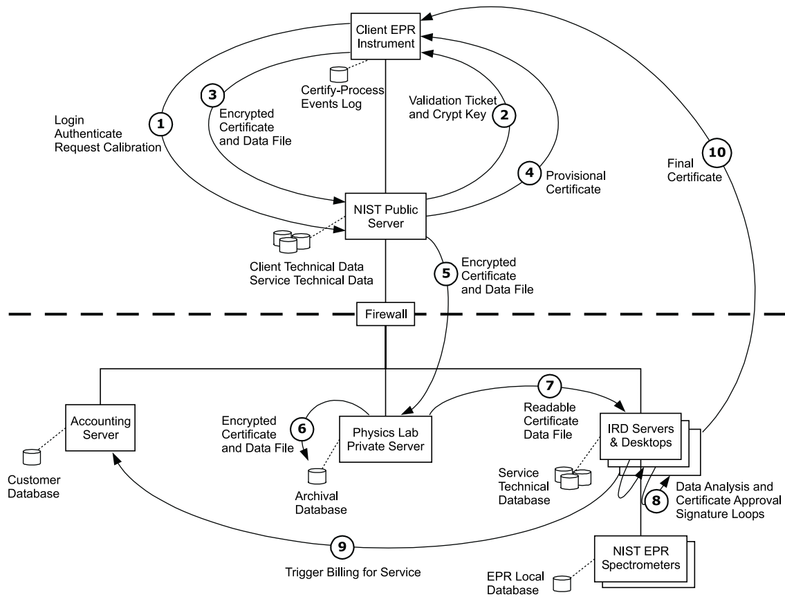
Figure 1. Hardware configuration and communication scheme for Internet-based certification service.
