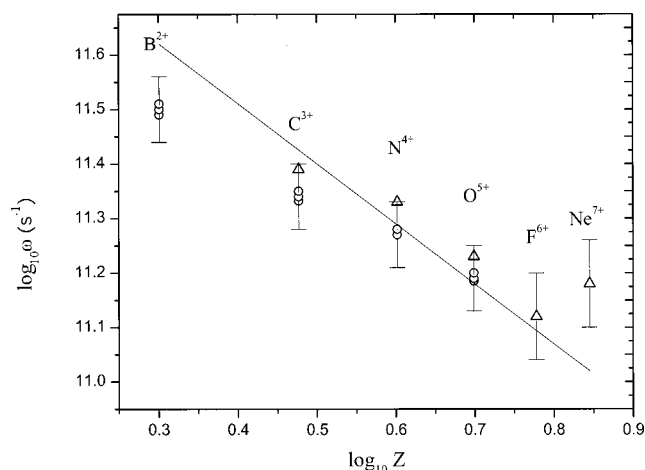
FIG. 1. Stark widths for the 3s^2S-3p^2P^o transition of lithium-like spectral lines (in units of angular frequency) as a function of \log_{10} Z according to Blagojević et al. 10 The experimental data are scaled linearly to a value of the electron density of 10^{17} \text{ e/cm}^3 and to an electron temperature value of 87 000 K (7.5 eV) using w_e(T_e) dependence from the theoretical data in Ref. 10. Experimental results: \Delta , Glenzer et al. ; 11 and \circ , Blagojević et al. 10 Error flags are calculated uncertainties including the error in the determination of the full width at half maximum and electron density measurements. The results of semiclassical calculations by Blagojević et al. , 10 shown for comparison, are given by the solid line.
