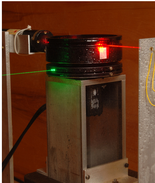
Figure 5 Photo of the Spinning Disk Unit.
