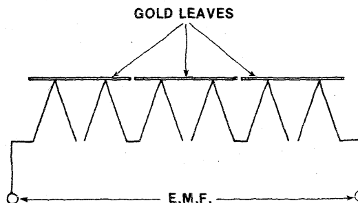
Figure 10—Schematic of thermopile detector.
