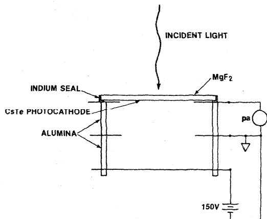
Figure 3—Schematic and wiring configuration of EVSD photodiode.
