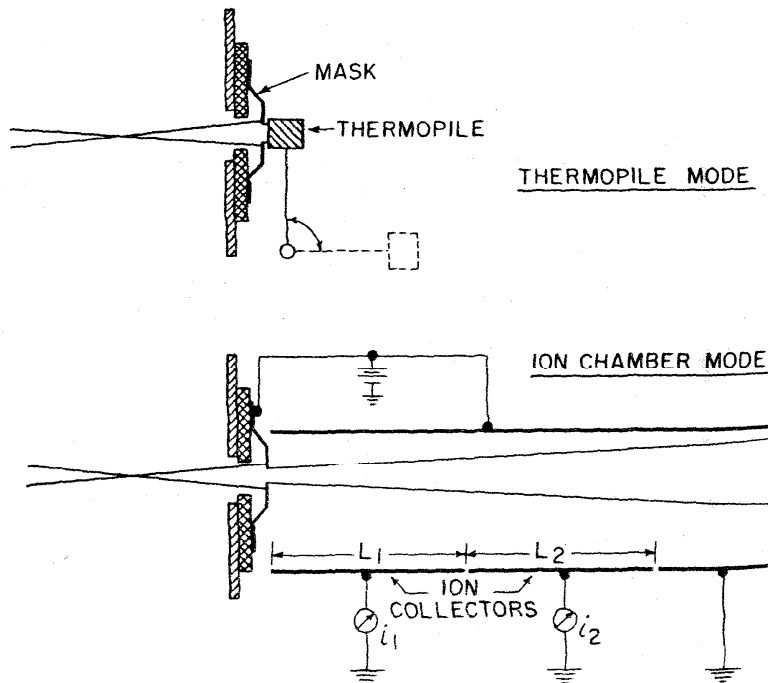
Figure 4—Configuration of thermopile and ionization chamber detectors.
