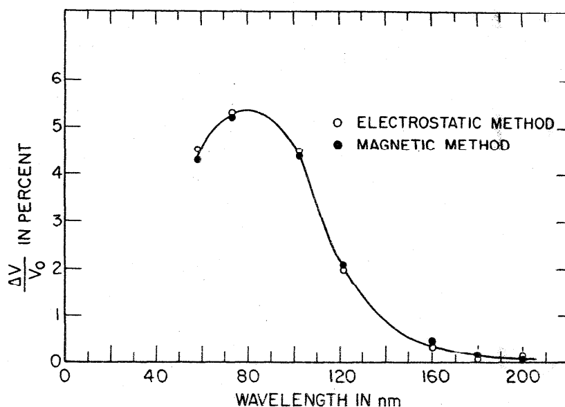
Figure 7—Wavelength dependence of thermopile signal loss due to photoejected electrons.
