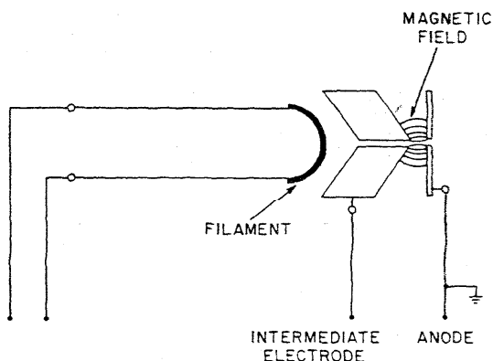
Figure 9—Duoplasmatron light source.
