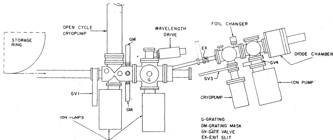
Figure 6—Detailed configuration of Far Ultraviolet Detector Facility at SURF-II
