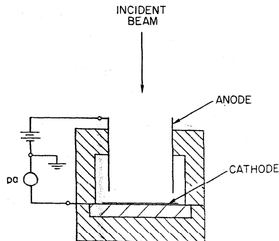
NBS PHOTODIODE (WINDOWLESS) (5-122 nm)
