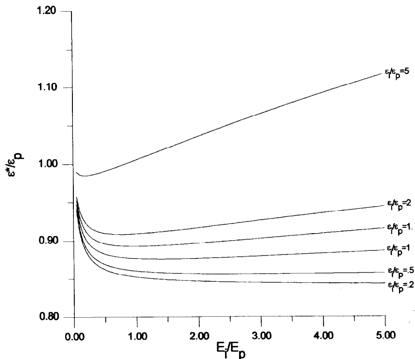
FIGURE 6. Three-dimensional analytical results for overall shrinkage at a sand area fraction of 5.9%.
