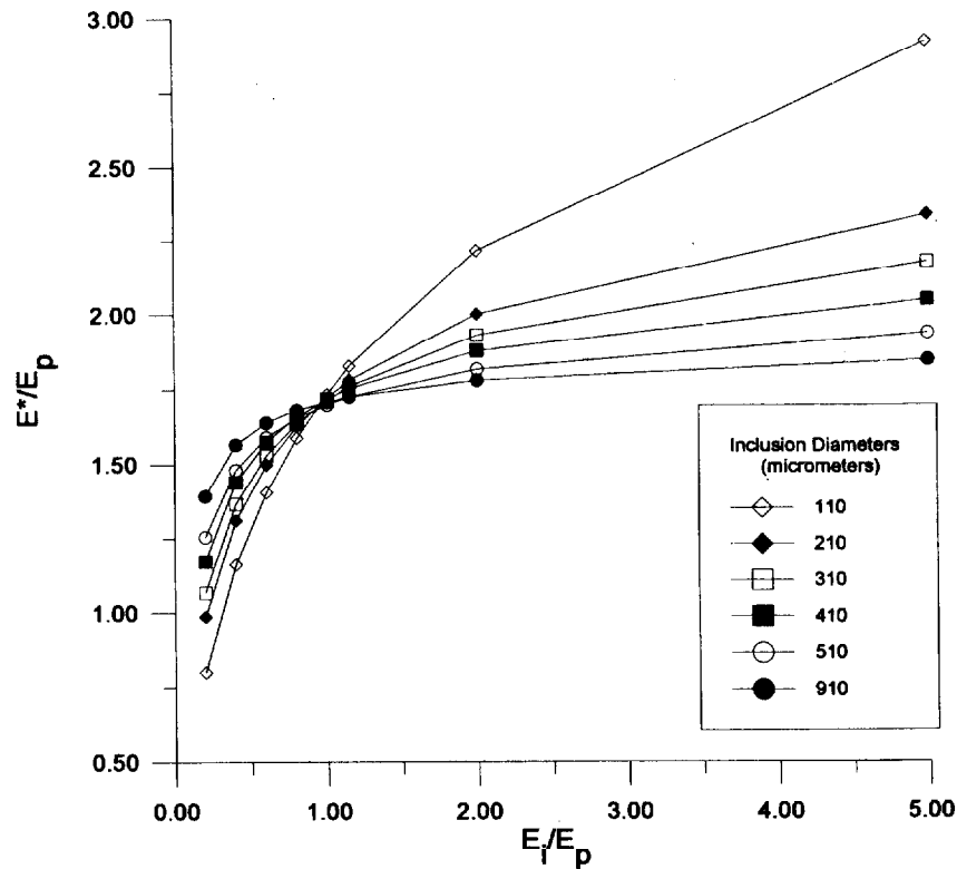
FIGURE 2. Effect of the ratio of the interfacial transition zone cement paste Young's modulus, E_i , to the bulk cement paste Young's modulus, E_p , on the composite Young's modulus, E^* , for different sand particle diameters at a constant area fraction of 55%.
