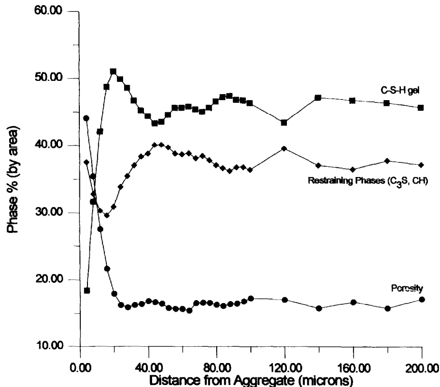
FIGURE 7. Phase volume fraction as determined by the cement paste microstructure model as a function of distance from an aggregate surface.
