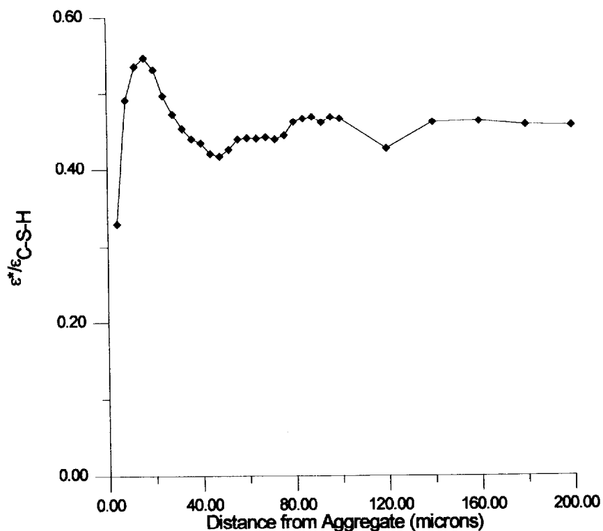
FIGURE 8. Overall shrinkage in the cement paste microstructure model as a function of distance from the aggregate surface.
