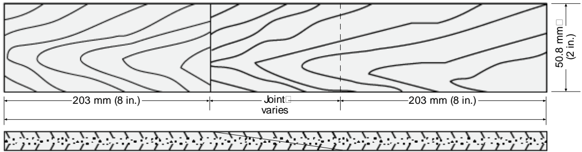
TENSION SPECIMEN FOR SCARFED JOINTED PANELS
