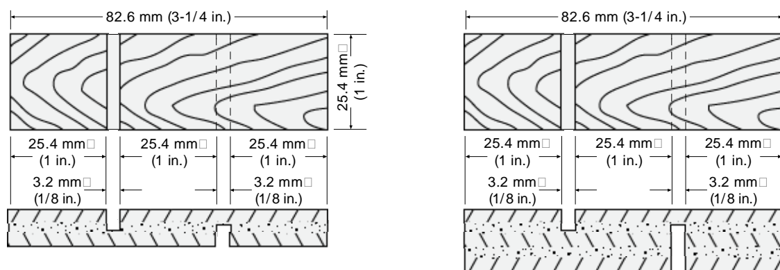
SHEAR TEST SPECIMENS
