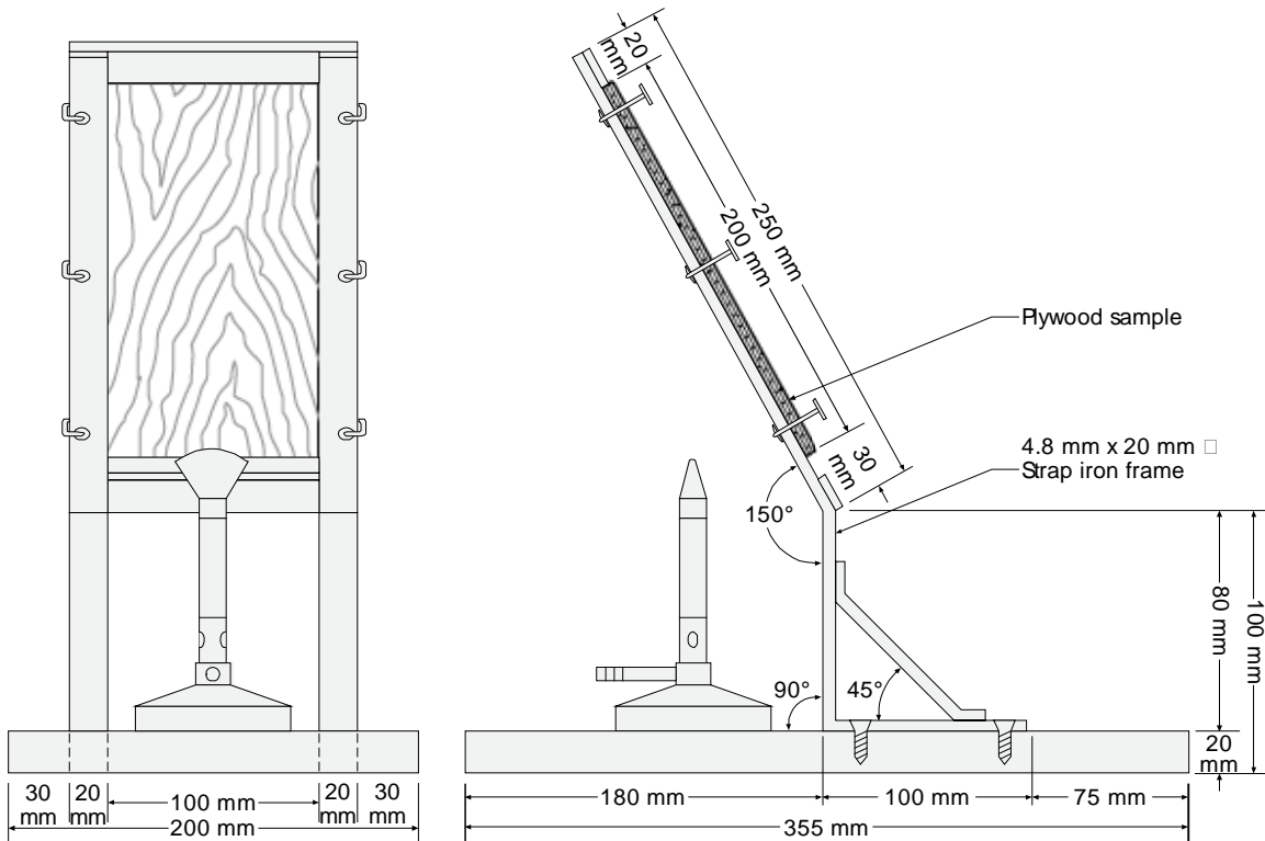
FIGURE 3 APPARATUS FOR HEAT DURABILITY TEST
