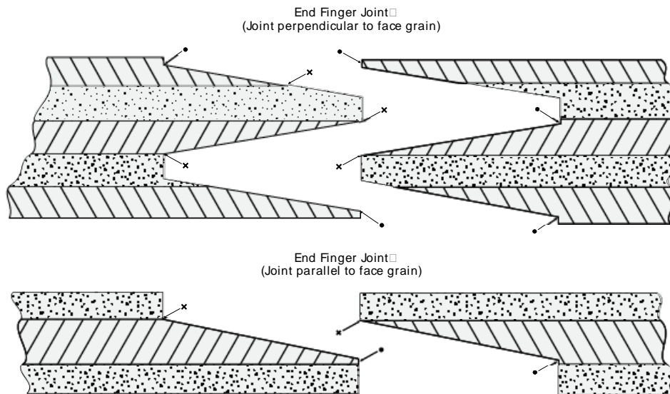
FINGER JOINTS – LOCATION OF SCARFED PORTION OF JOINTS
