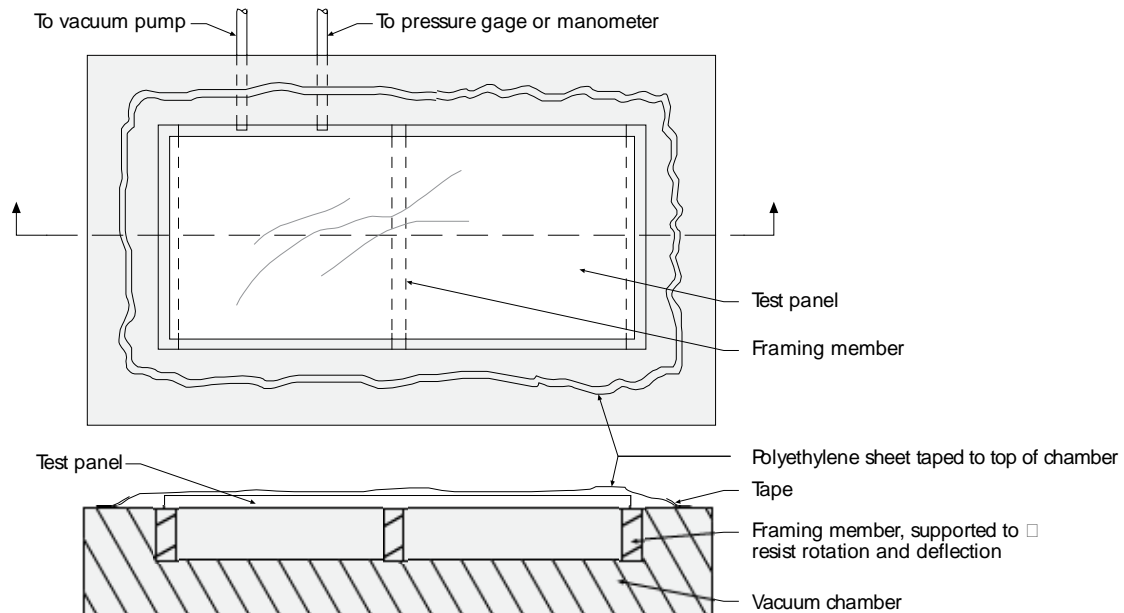
VACUUM CHAMBER TEST EQUIPMENT
