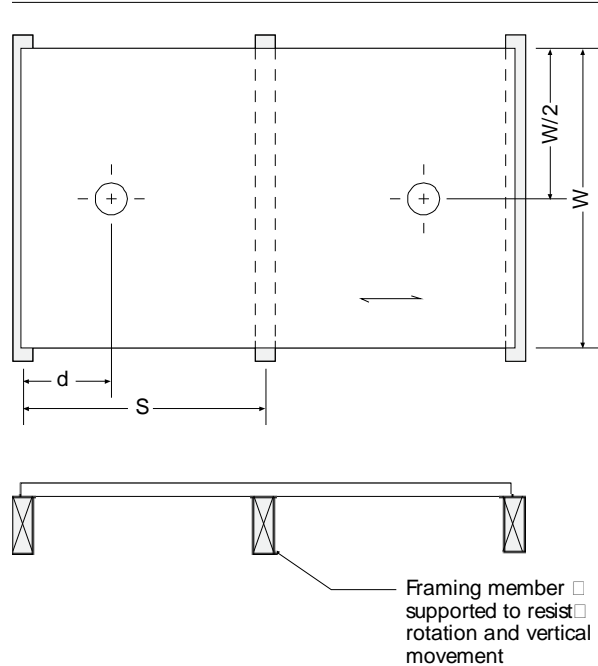
UNIFORM-LOAD TEST SPECIMENS
