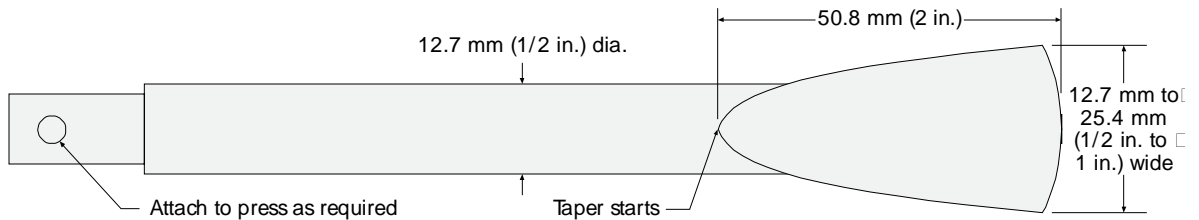
WEDGE OR CHISEL USED FOR CLEAVAGE TEST
