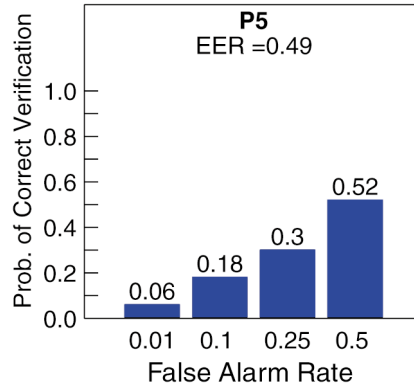
Figure 48: FRVT 2000 Pose Experiments—C-VIS Verification Scores
