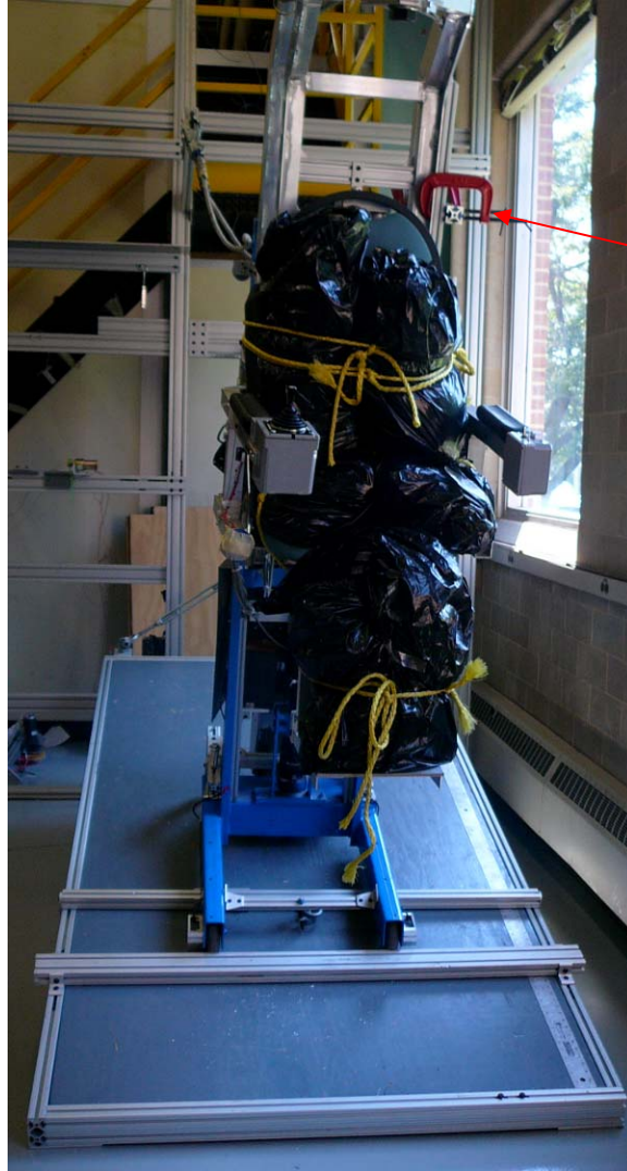
Figure 12. Seat Height High Seat Forward Orientation
