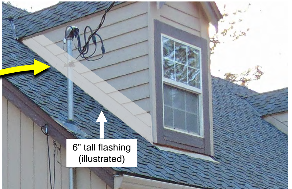
Item 3.2 Roof Assembly Details (Dormers) – Flashing and ignition resistant siding to protect dormer from ignition by combustible debris and embers.
