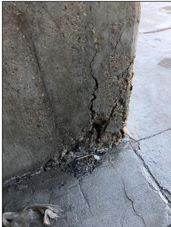
Photo C-162. Spall at Rusted Rebar
