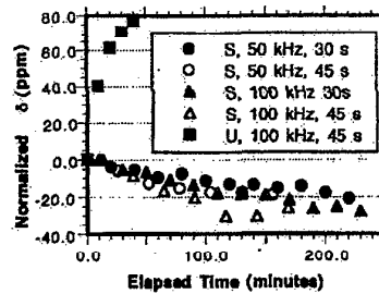
Fig. 3. Ac-dc differences as a function of warmup time for various resistors at different frequencies and delay times. Voltage (600 V on a 600-V range) was applied to the NIST standard HVTC at t = 0 in the plot. After a one-hour warmup, the test HVTC was connected and measurements made as it warmed from room temperature. In the legend, S indicates an internal shield was present, and U indicates the absence of an internal shield. The resistors were untreated in all cases.
