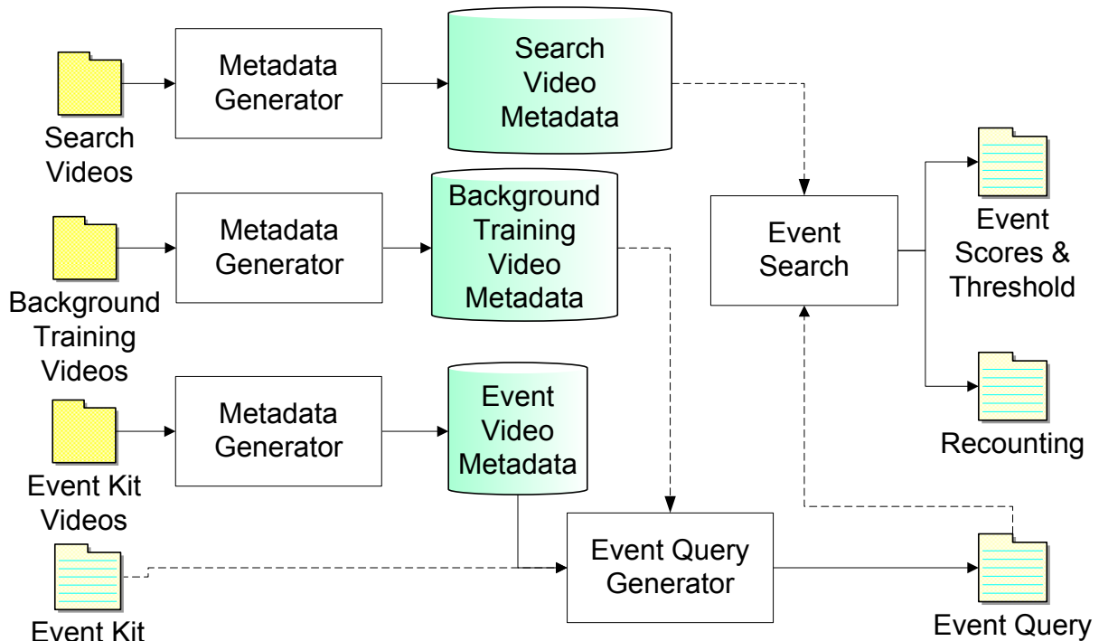
Figure 1: MED System Block Diagram: The MED processing modules are shown in blocks and data is depicted as icons. Folder icons represent a collection of videos while text-folders are text/csv documents. Dashed lines in the diagram show that significant time can elapse between the computation of the data and its use in the following module.
