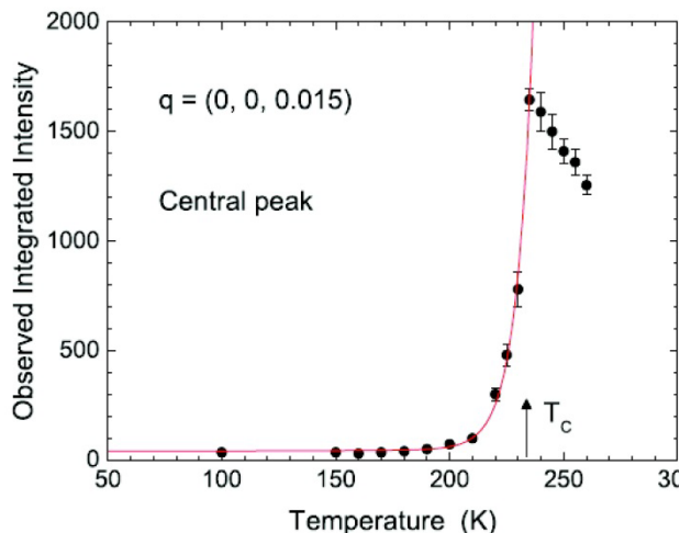
Intensity of the quasielastic peak for \text{La}_{0.85}\text{Sr}_{0.15}\text{MnO}_3 at (0\ 0\ 0.15) as a function of temperature [4].
