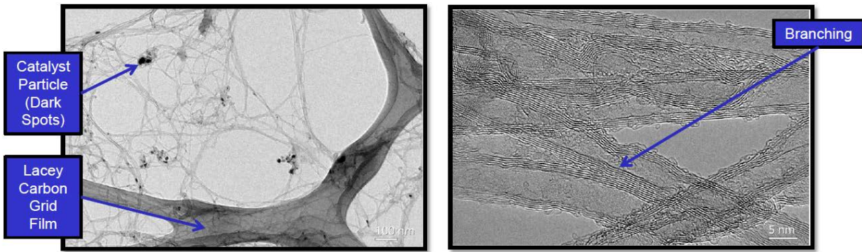
Figure 3. Transmission electron microscope images of CNT networks (from presentation by Tushar Shah, Applied Nanostructured Solutions).
