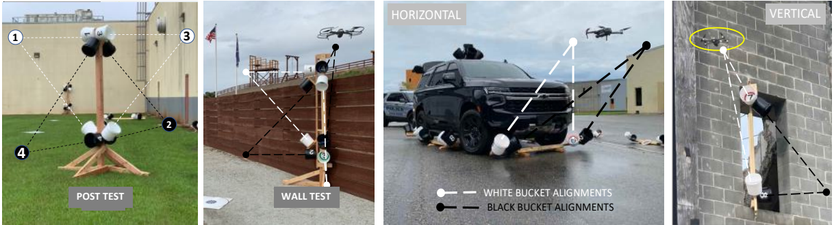
Dual Bucket Alignments Guide Remote Pilots to Safe Positions in Proximity to Objects
