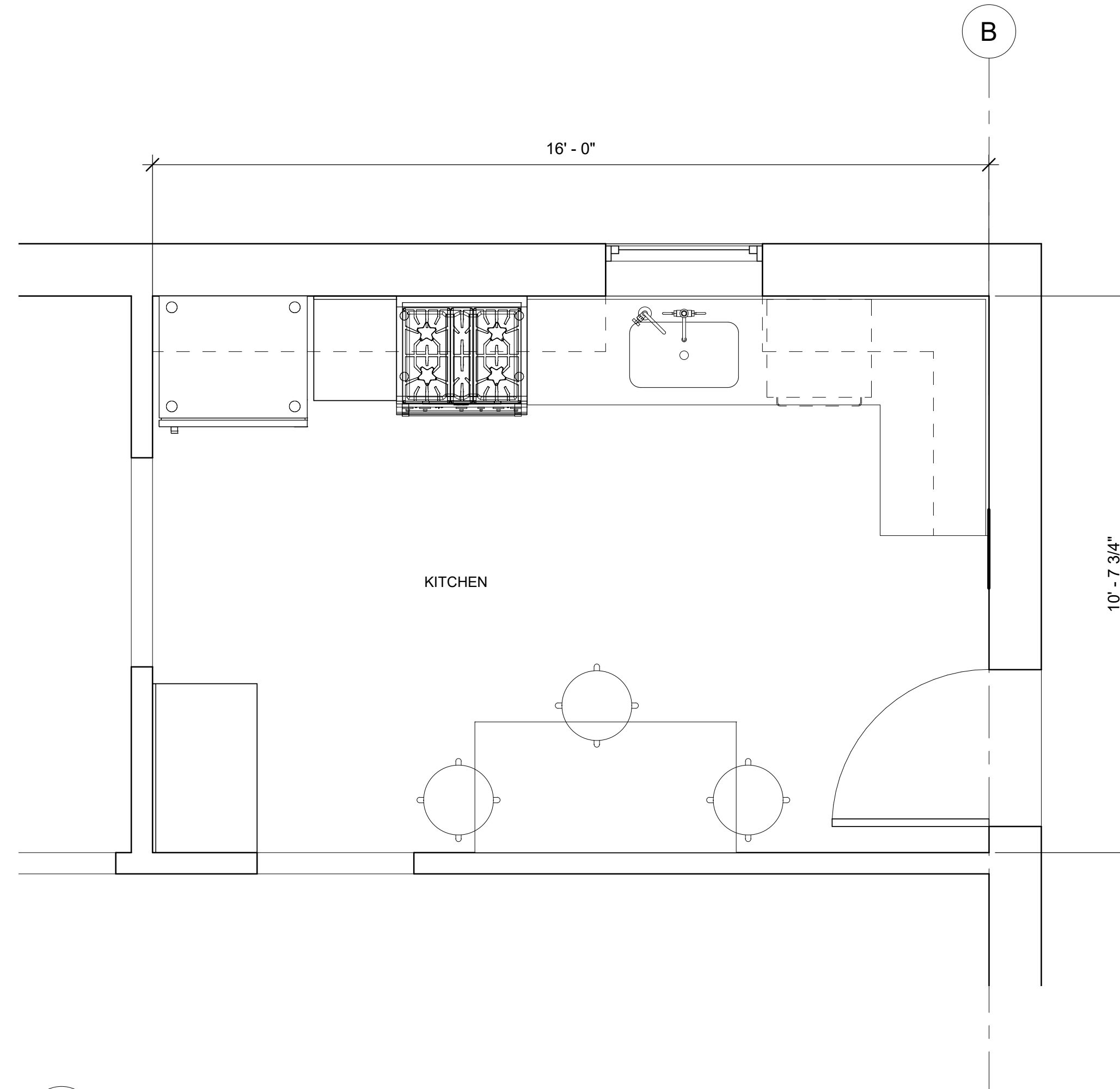
32 FIRST FLOOR PLAN KITCHEN LAYOUT A-101 1/2" = 1'-0"
