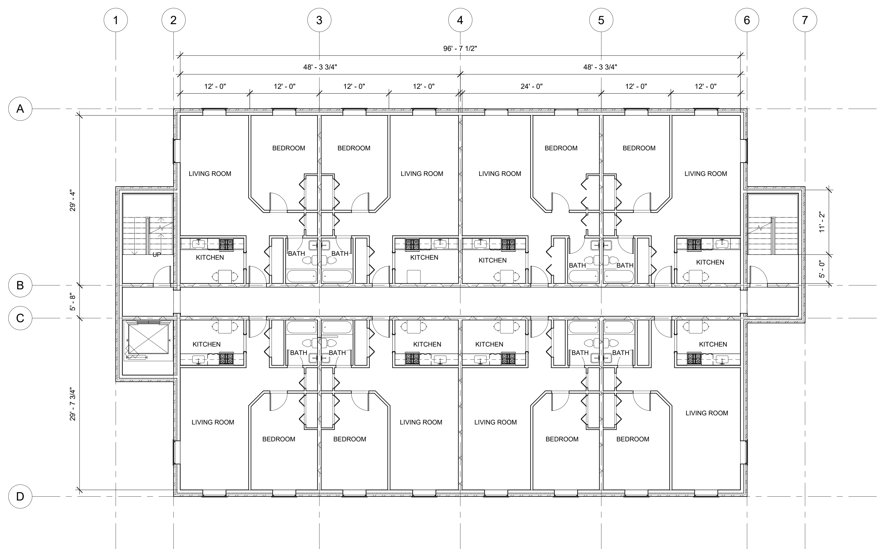
41 SECOND FLOOR PLAN A-301 1/8" = 1'-0"
