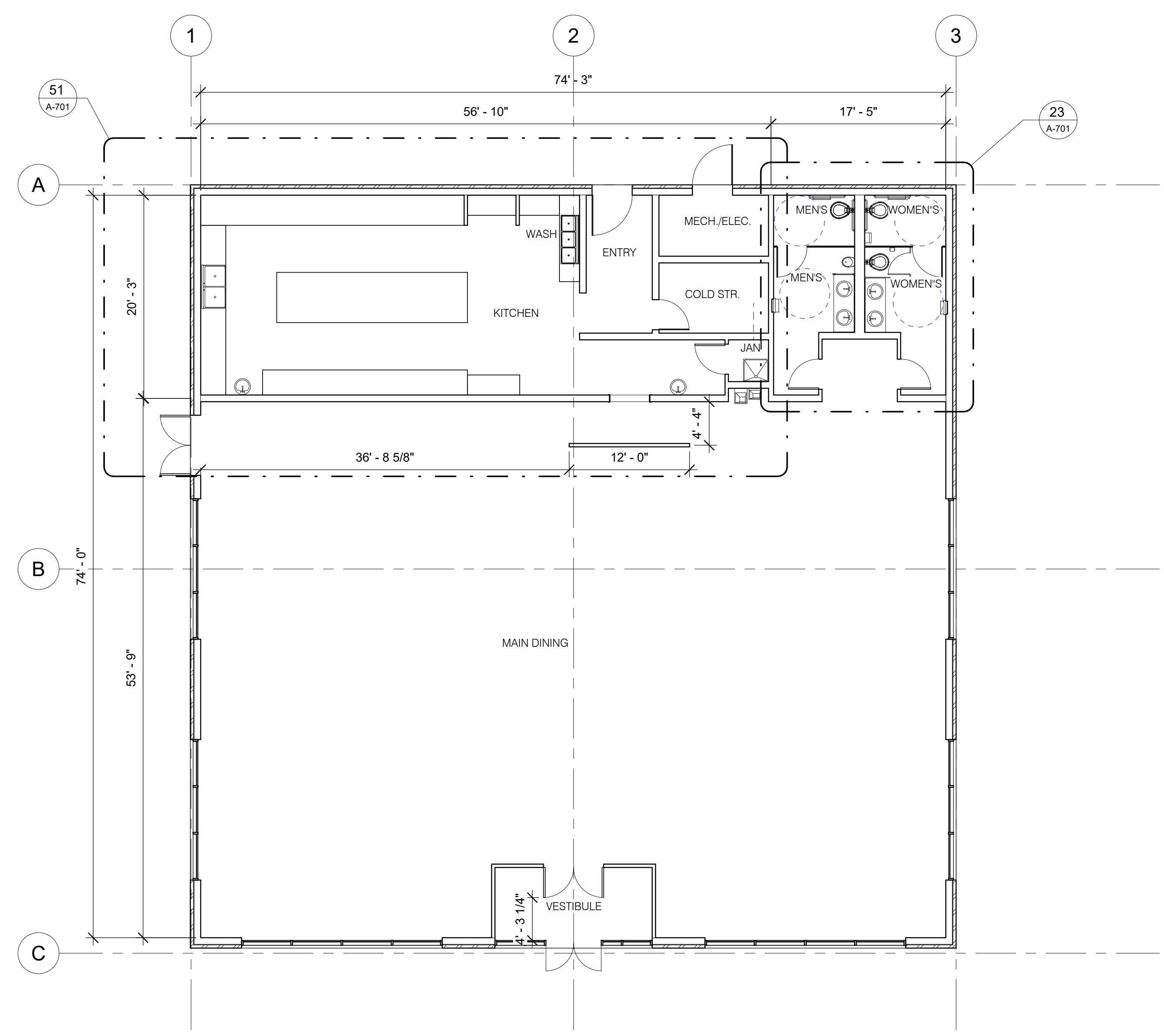
21 FIRST FLOOR PLAN A-701 1/8" = 1'-0"
