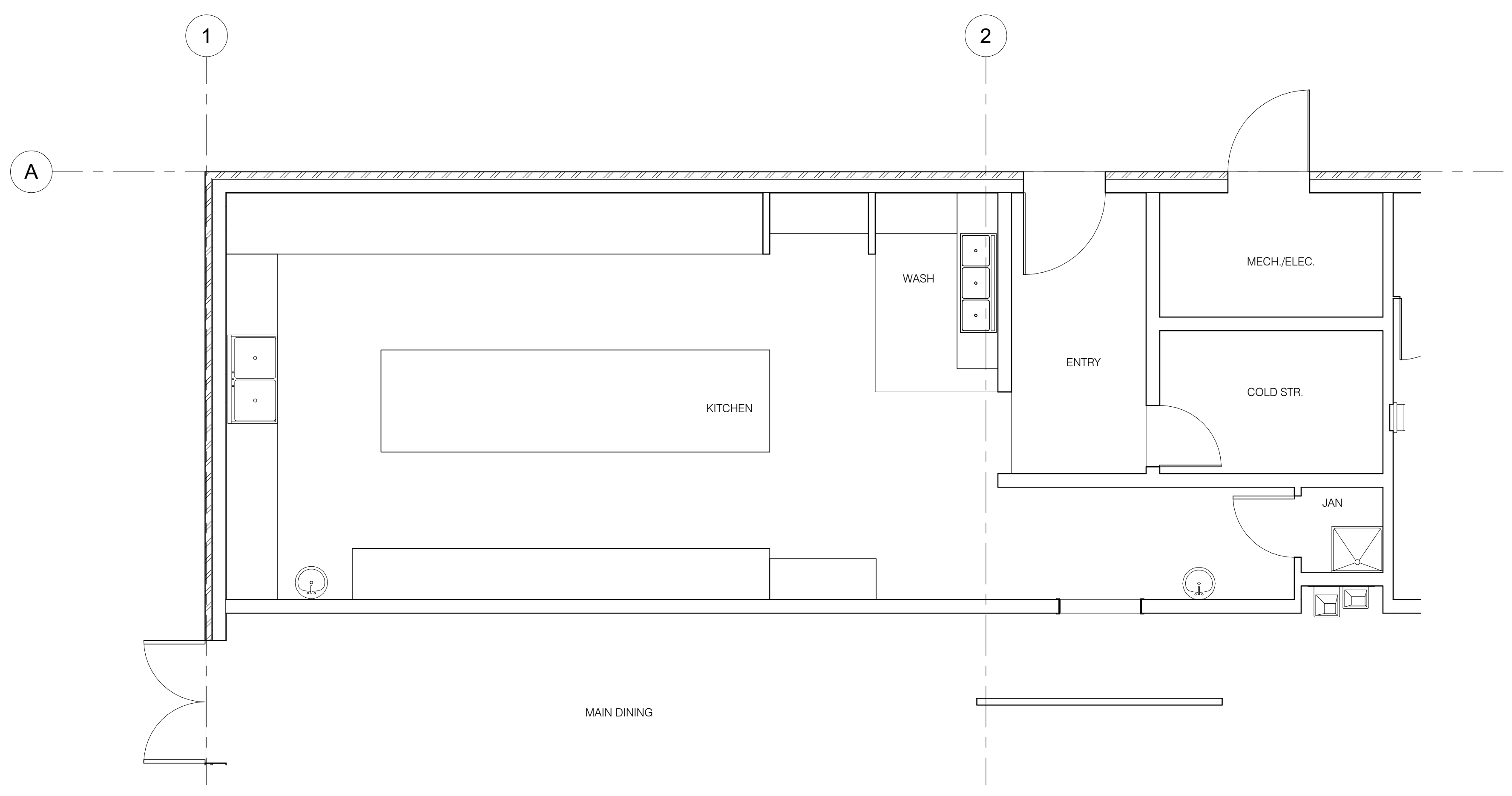
51 KITCHEN FLOOR PLAN - ENLARGED A-701 1/4" = 1'-0"
