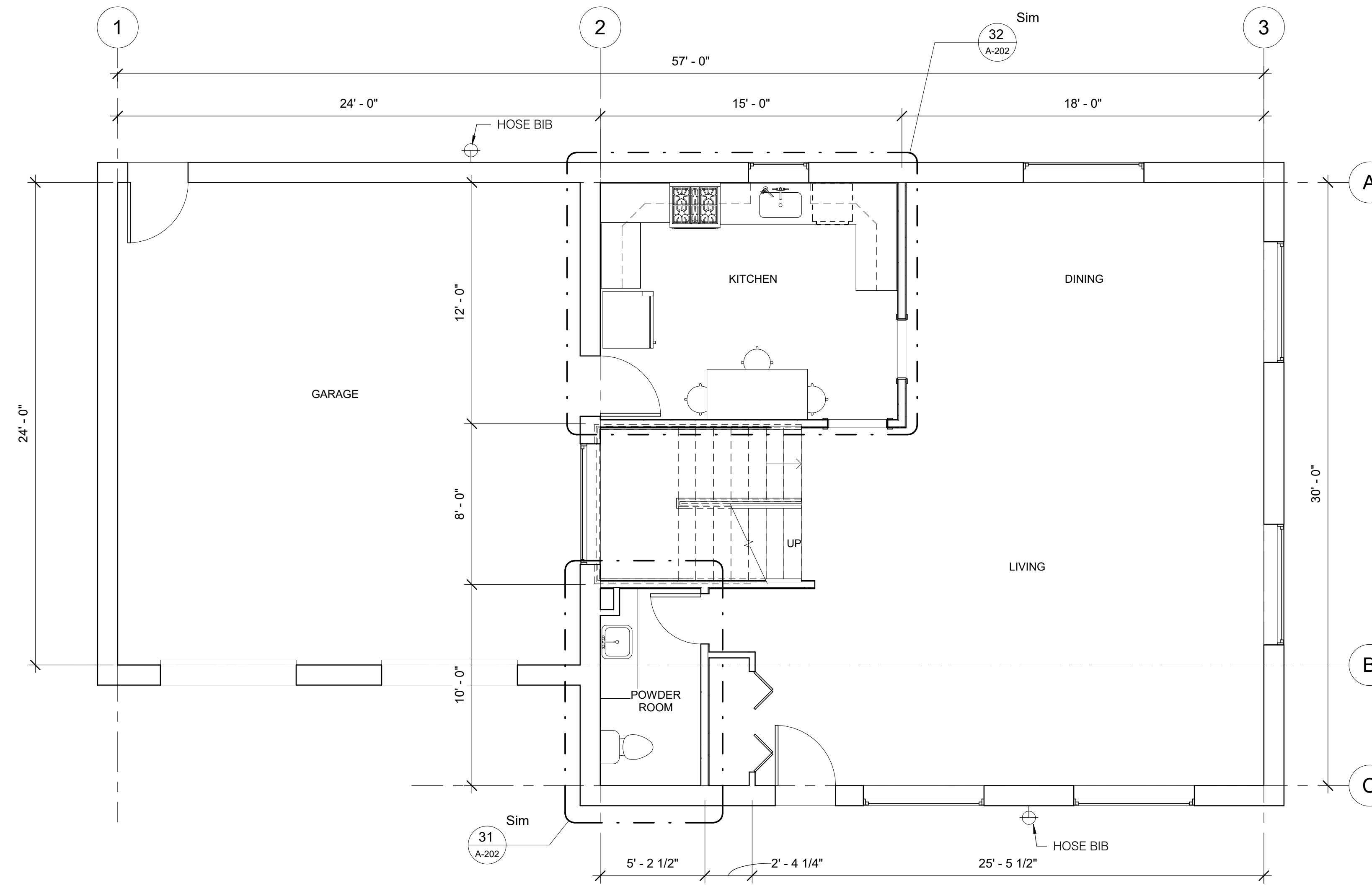
23 FIRST FLOOR PLAN A-201 1/4" = 1'-0"
