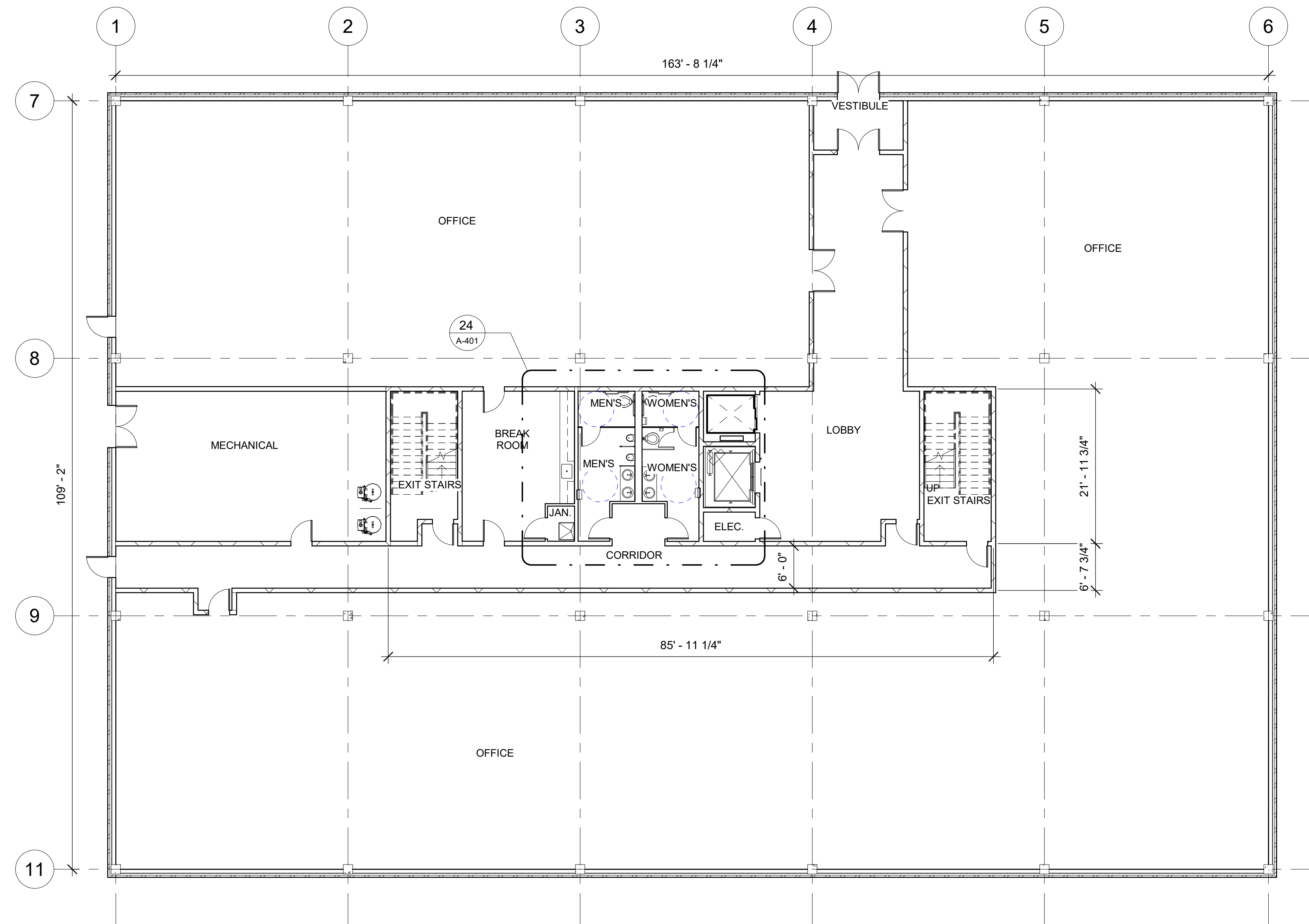
21 FIRST FLOOR PLAN A-401 3/32" = 1'-0"
