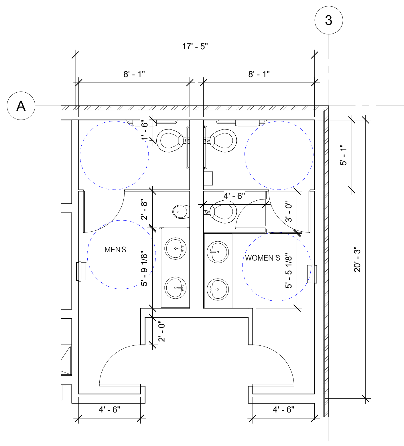
23 RESTROOM FLOOR PLAN - ENLARGED A-701 1/4" = 1'-0"
