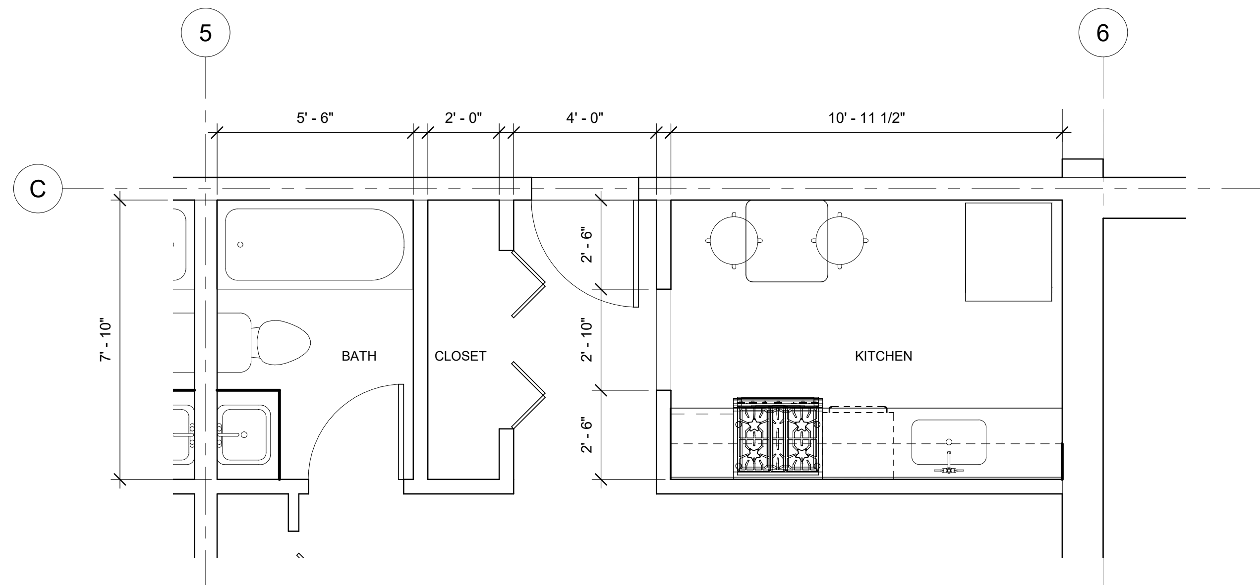
44 KITCHEN AND RESTROOM LAYOUT (TYPICAL) A-301 3/8" = 1'-0"
