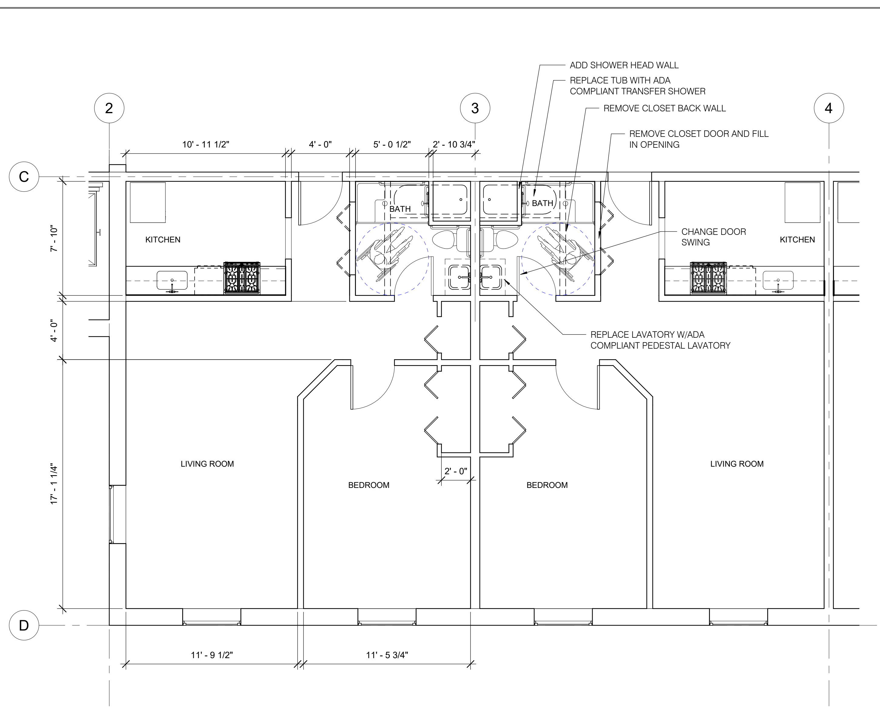
24 ADA ADAPTABLE UNIT LAYOUT A-301 1/4" = 1'-0"
