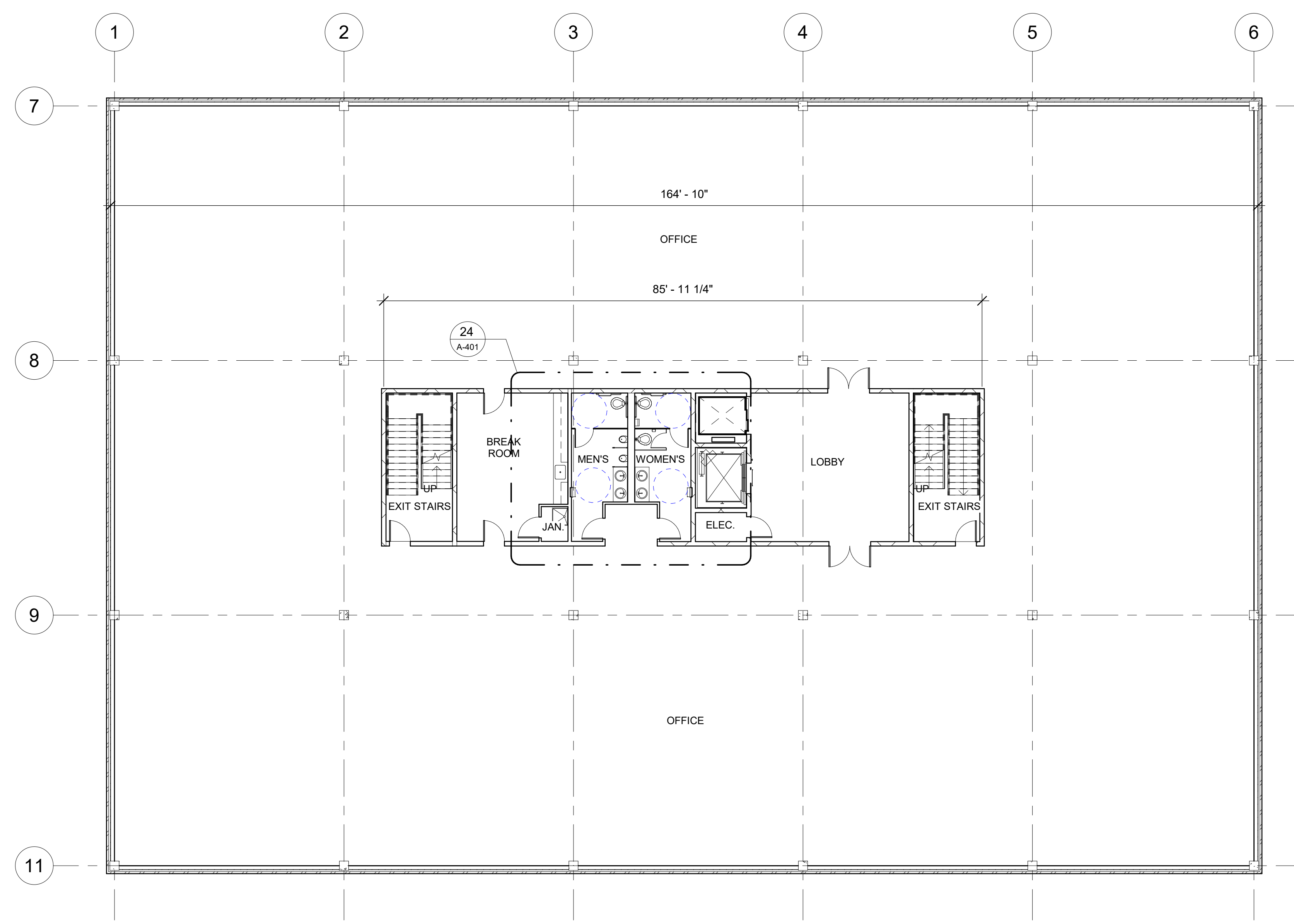
41 SECOND AND THIRD FLOOR PLAN (TYPICAL) A-401 3/32" = 1'-0"
