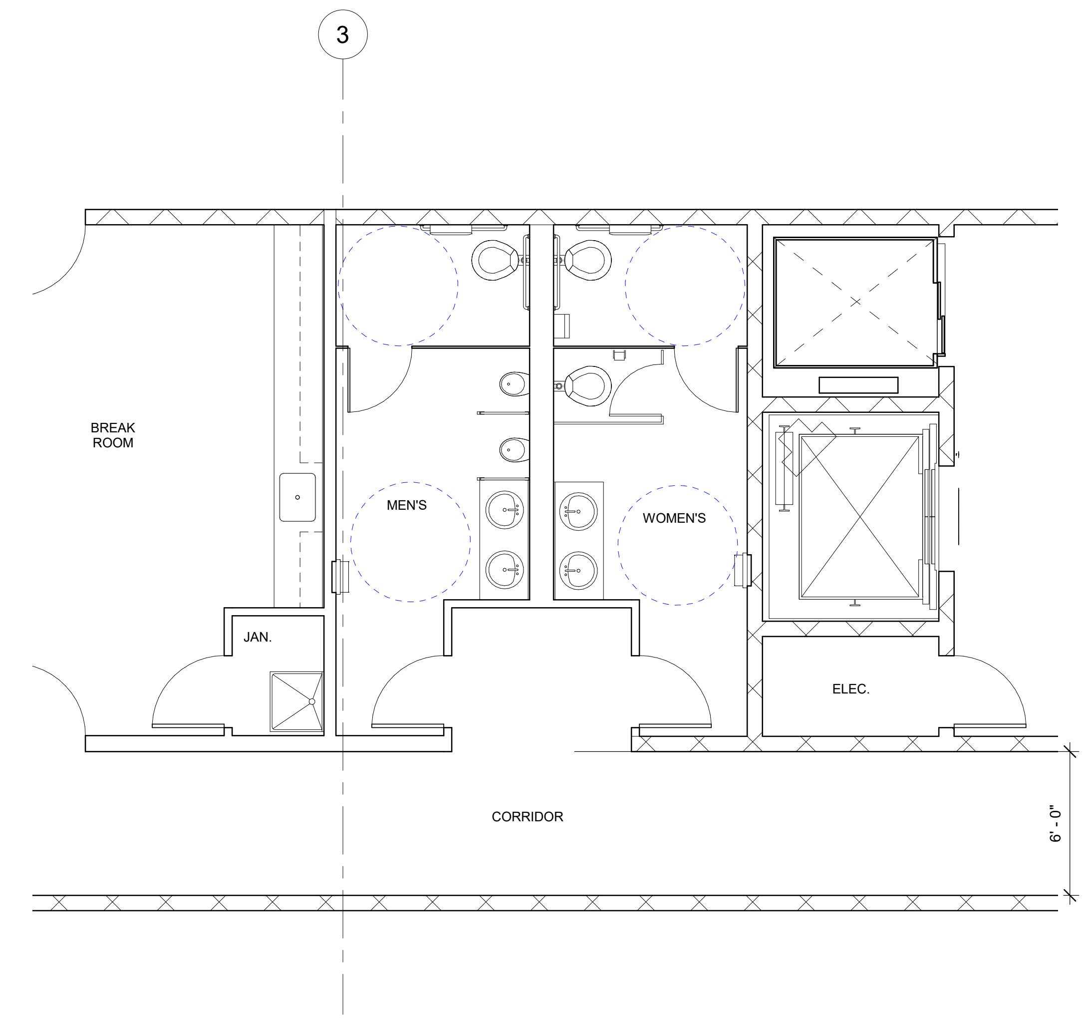
24 ENLARGED RESTROOM LAYOUT A-401 1/4" = 1'-0"
