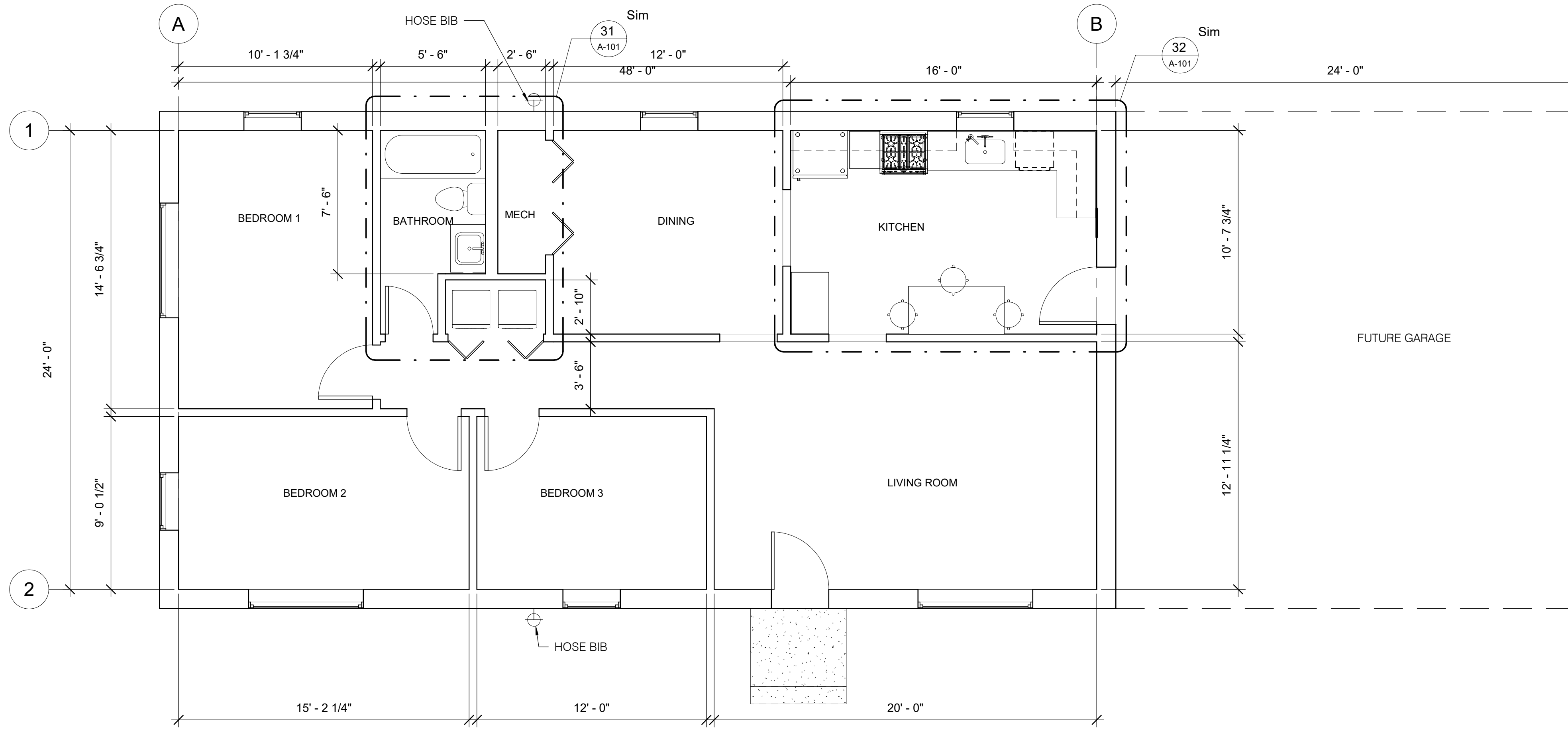
21 FIRST FLOOR PLAN A-101 1/4" = 1'-0"
