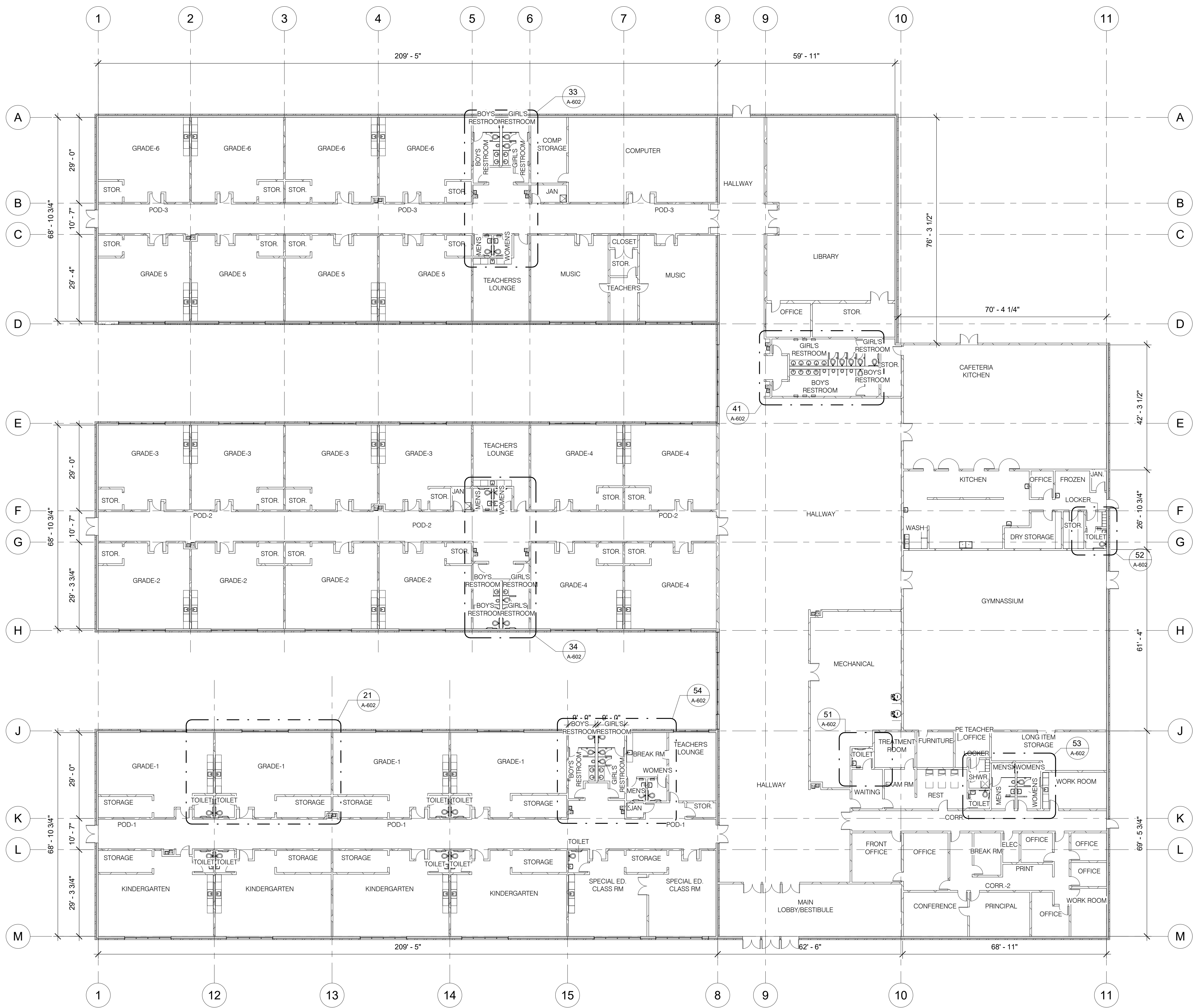
1 FIRST FLOOR PLAN A-601 1/16" = 1'-0"
