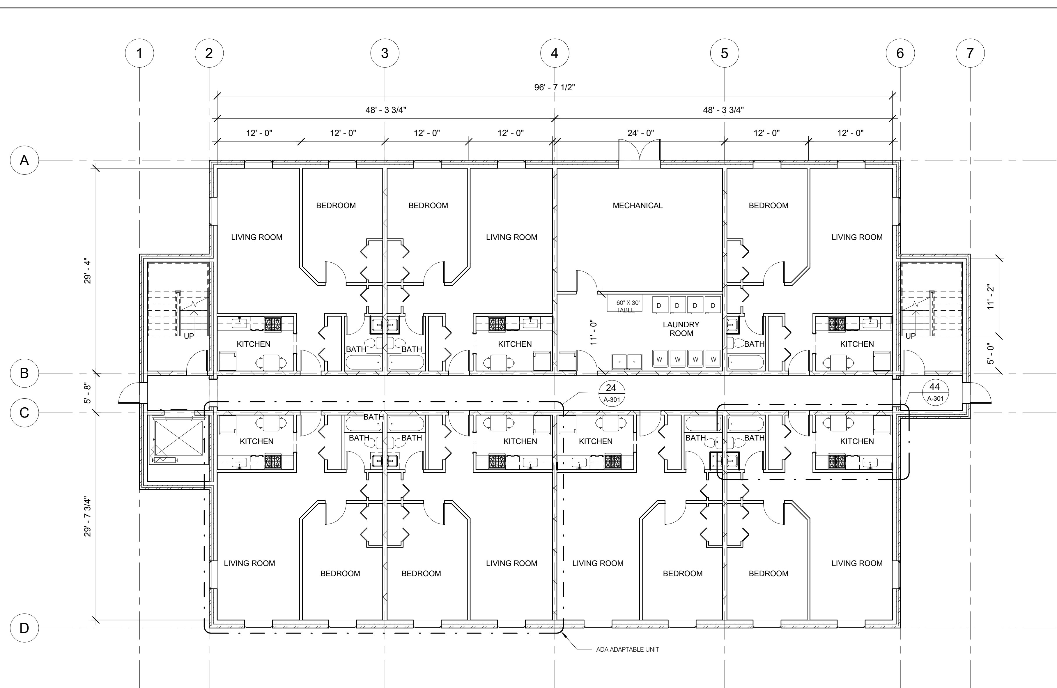
21 FIRST FLOOR PLAN A-301 1/8" = 1'-0"
