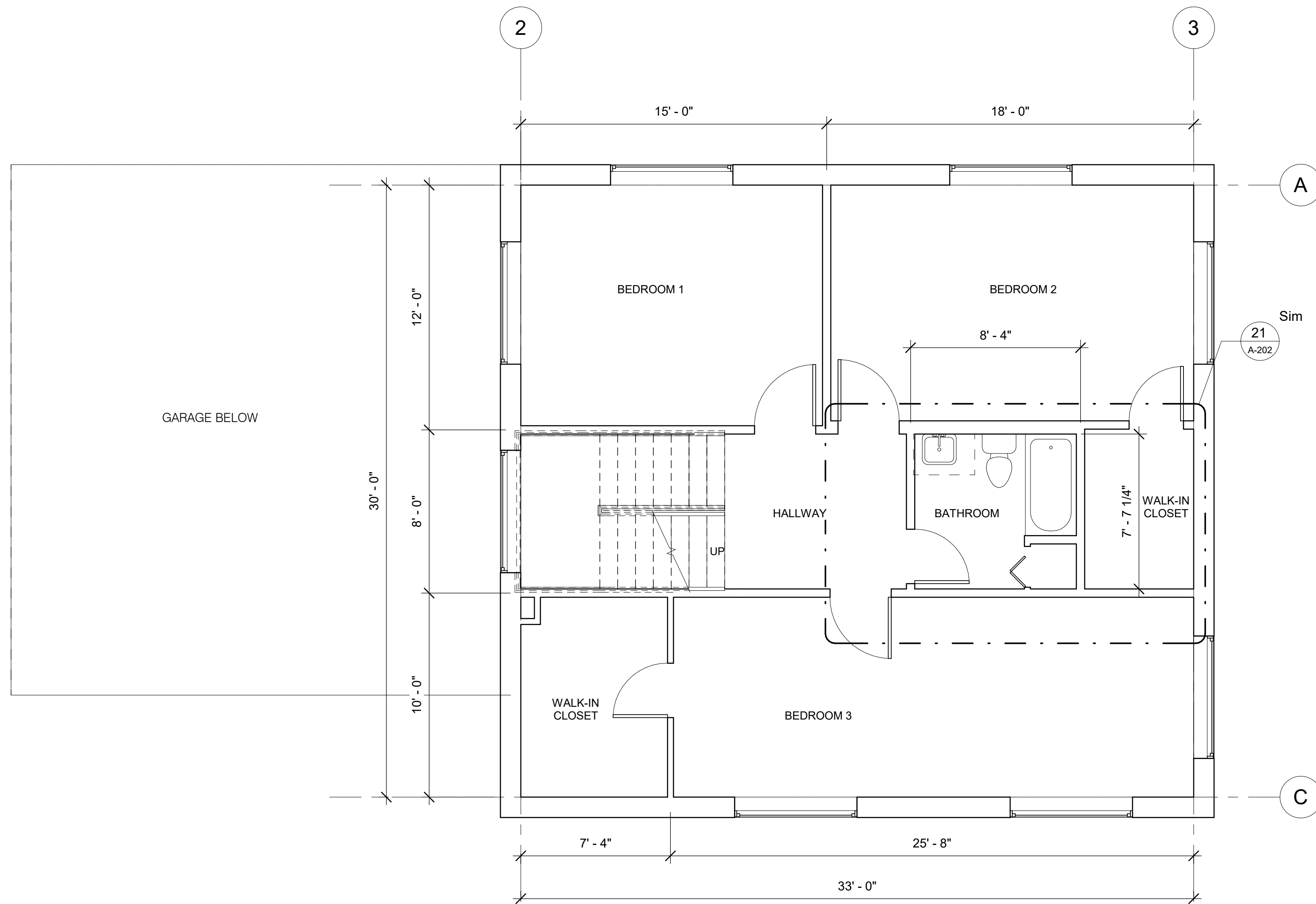
21 SECOND FLOOR PLAN A-201 1/4" = 1'-0"
