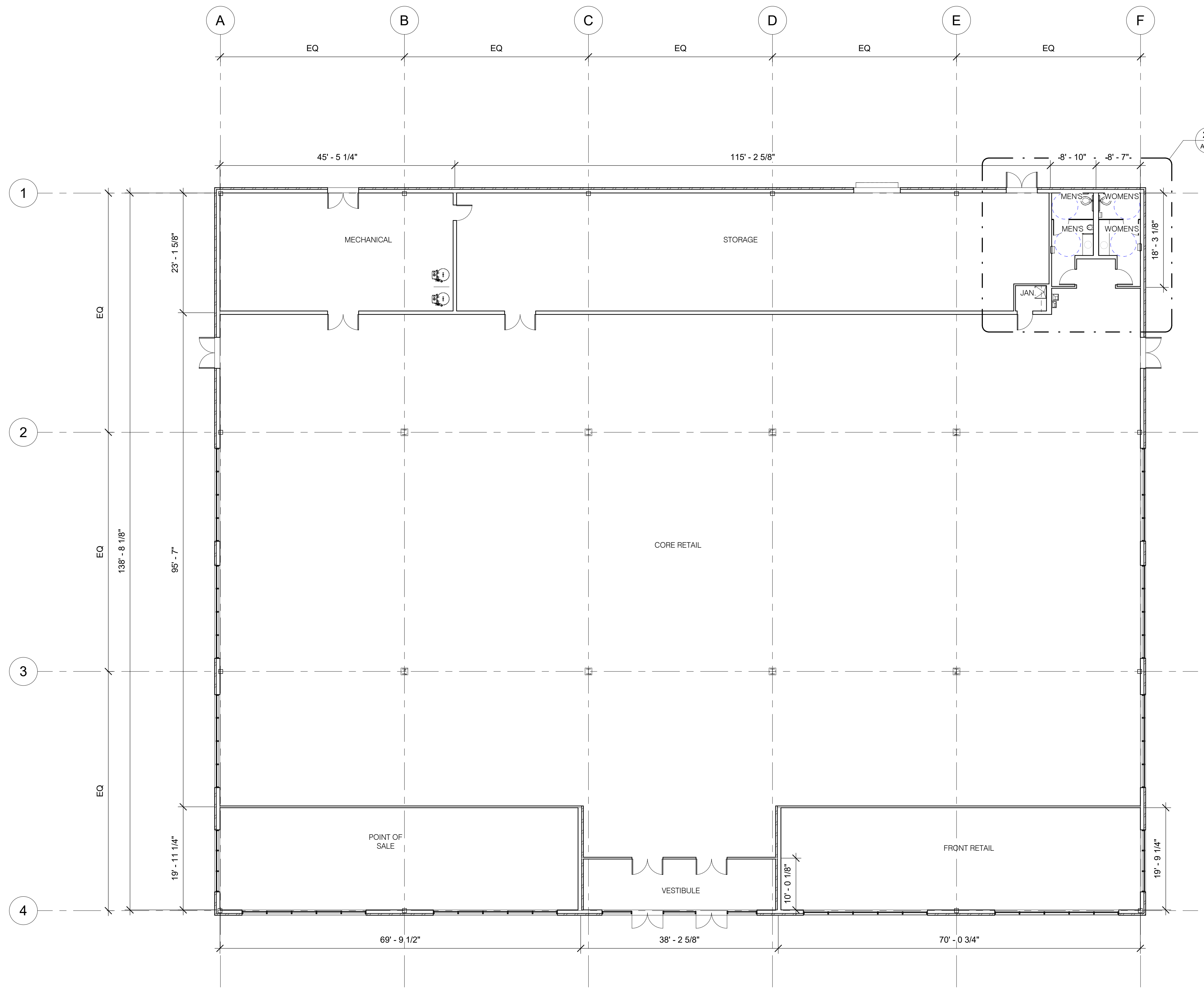
31 FIRST FLOOR PLAN A-501 3/32" = 1'-0"
