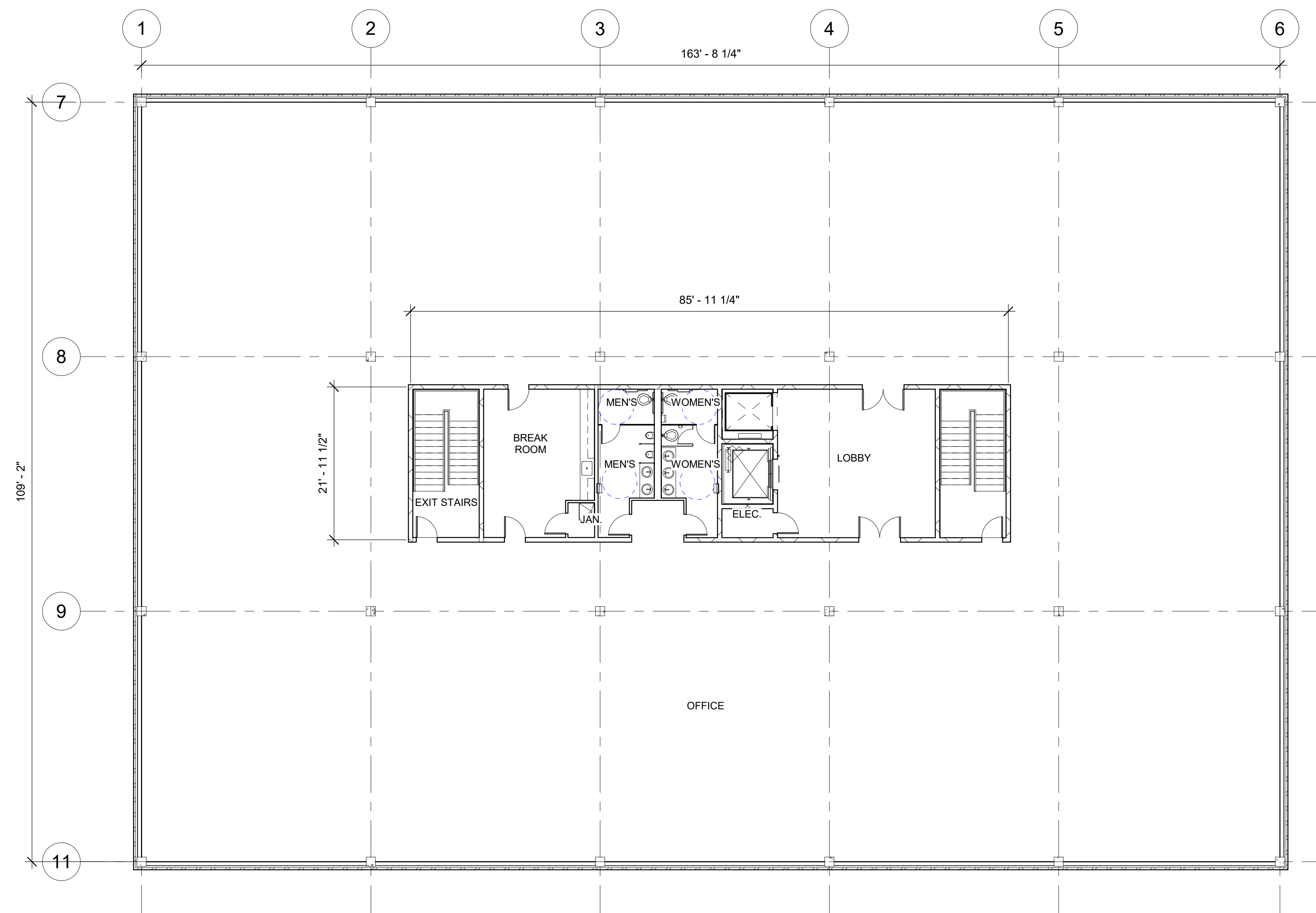
21 THIRD FLOOR PLAN A-402 3/32" = 1'-0"
