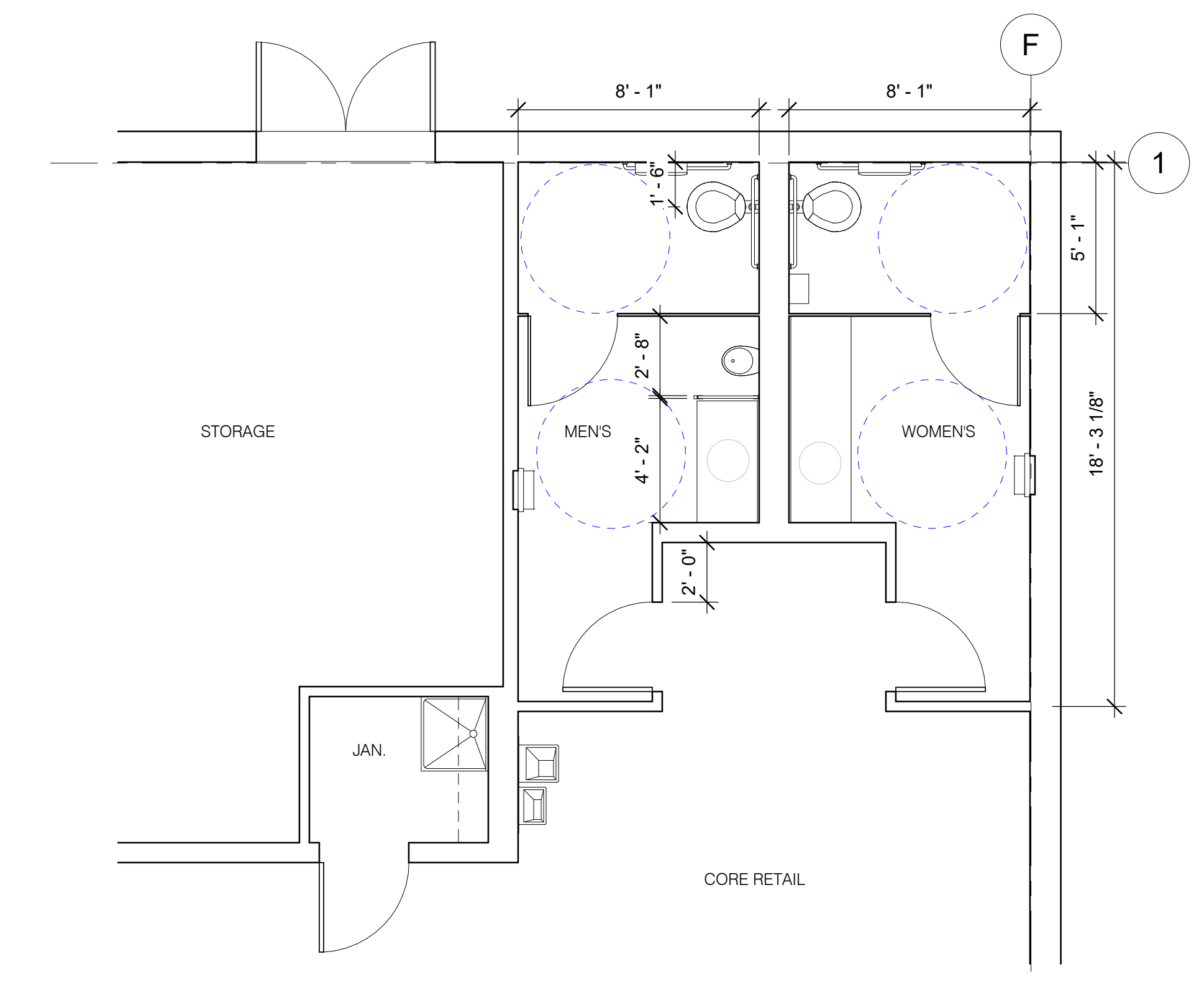
24 RESTROOM LAYOUT A-501 1/4" = 1'-0"
