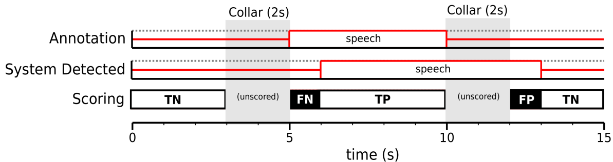
Figure 1: After collar application, systems are not scored on false alarms within two seconds from speech boundaries.
