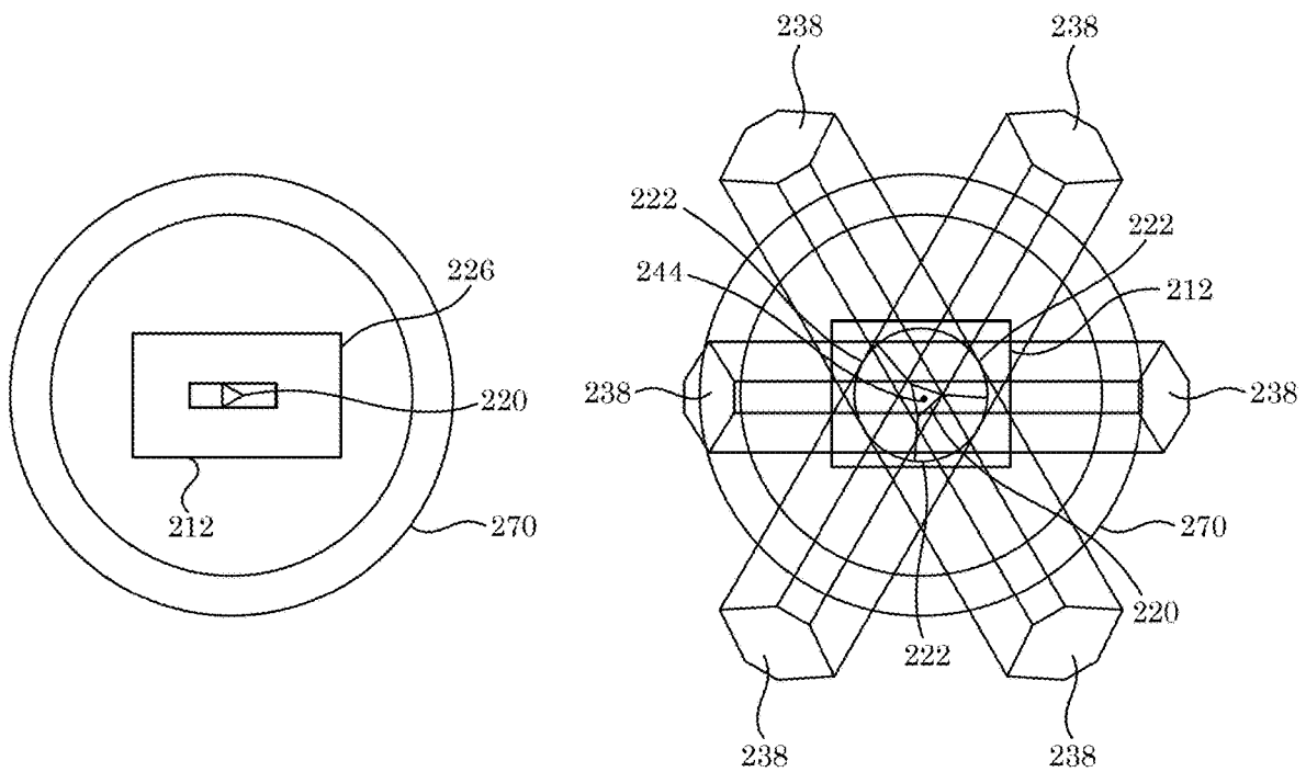
Bottom View
