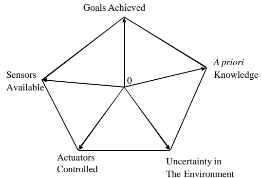
Figure 6 – Generalization of Figure 5 to now Include 5 Attributes
