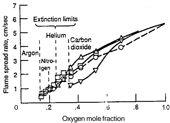
Figure 6.—Experimental flame spread rates for 0.076 mm thick paper under different oxygen-diluent atmospheres. Quantities are microgravity conditions with oxygen quantity fixed at 21 kPa partial pressure (air value).
