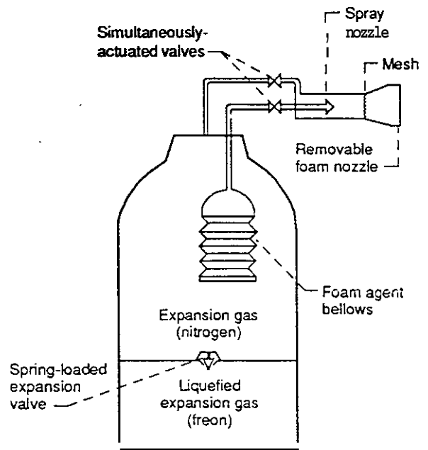
Figure 2.—Apollo Skylab foam fire extinguisher.
