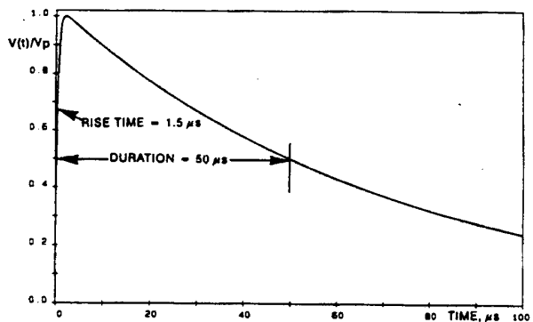
Combination Wave, Open-Circuit Voltage
