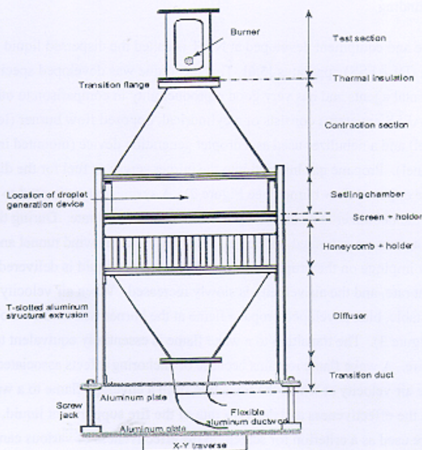
Figure 2. Schematic Representation of the DLAFFS Apparatus.
