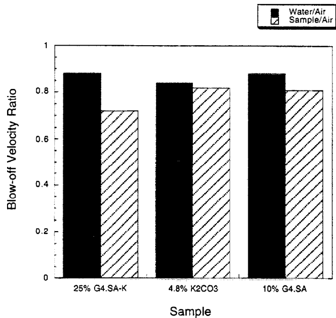
Figure 10. Blow-off Velocity Ratios for Various Candidate Agents to Air, and Reference Ratios for Water to Air Measured With the Same Conditions (pump rate of suppressant fluid to nebulizer is 0.3 ml/min in all cases).
