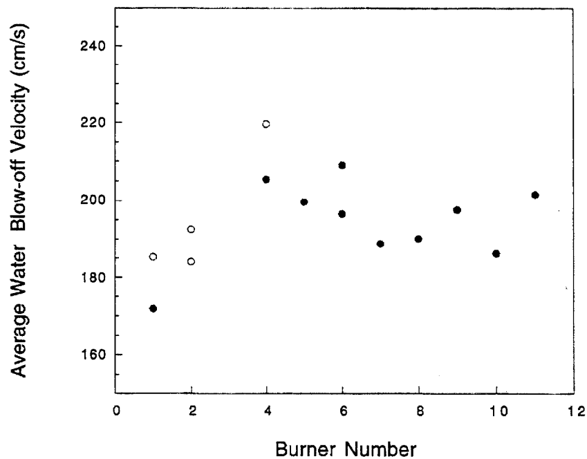
Figure 8. Average Water Blow-Off Velocity Recorded Using Different Propane Burners (all values taken on a given day using a given burner were included in the arithmetic average; open circles, water pumped to nebulizer at 0.3 ml/min; closed circles, water pumped to nebulizer at 0.5 ml/min).
