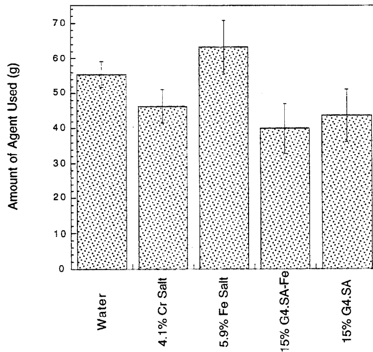
Figure 13. Amount of Various Experimental Fire Suppression Agents Required to Extinguish a 200-ml JP8 Fuel Pan Fire (error bars represent \pm 1 standard deviation).
