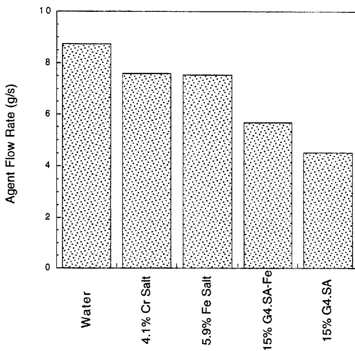
Figure 14. Mass Flow Rates for Various Experimental Fire Suppression Agents Deployed During JP8 Fire Suppression Agent Screening Experiments.
