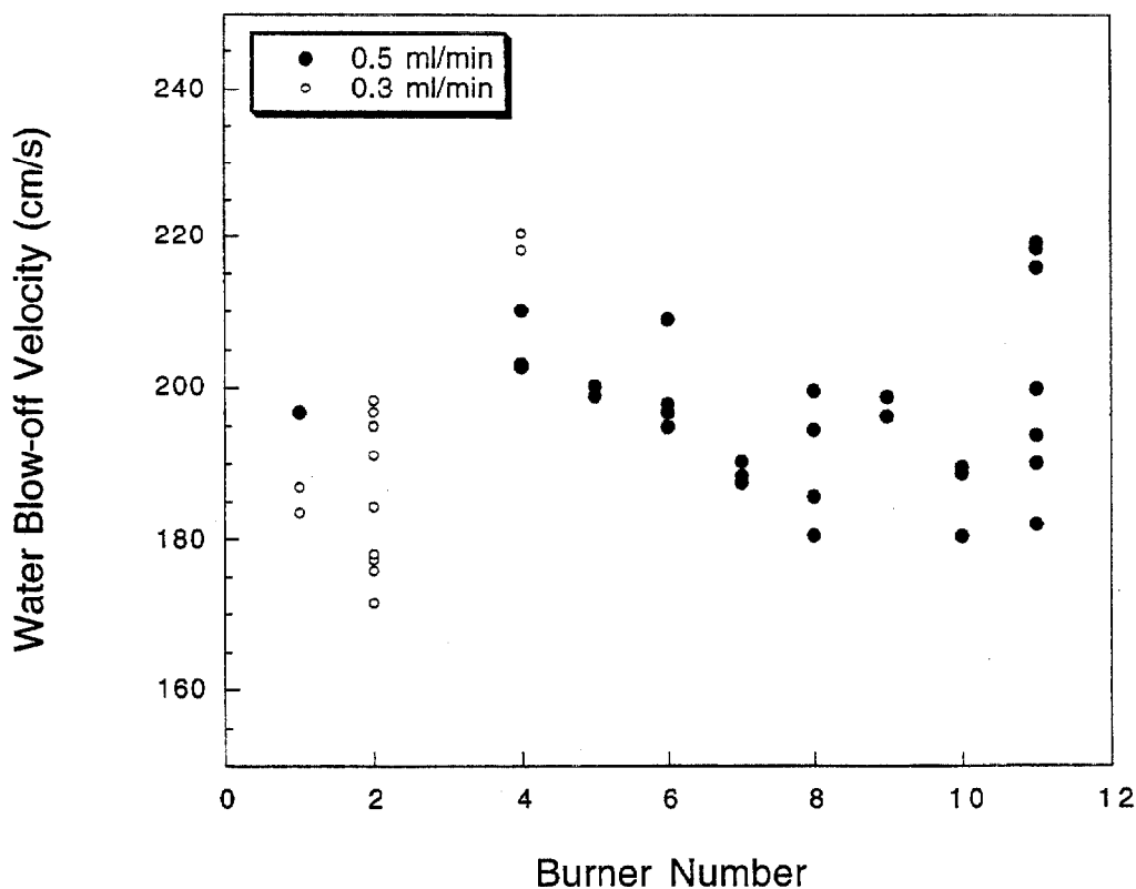
Figure 6. Water Blow-off Velocity Recorded Using Different Propane Burner Elements (open circles, water pumped to nebulizer at 0.3 ml/min; closed circles, water pumped to nebulizer at 0.5 ml/min).
