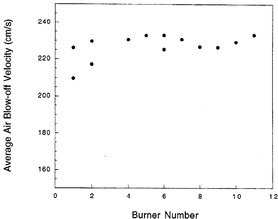
Figure 7. Average Air Blow-Off Velocity Recorded Using Different Propane Burners (all values collected using a given burner on a given day were included in the arithmetic average).
