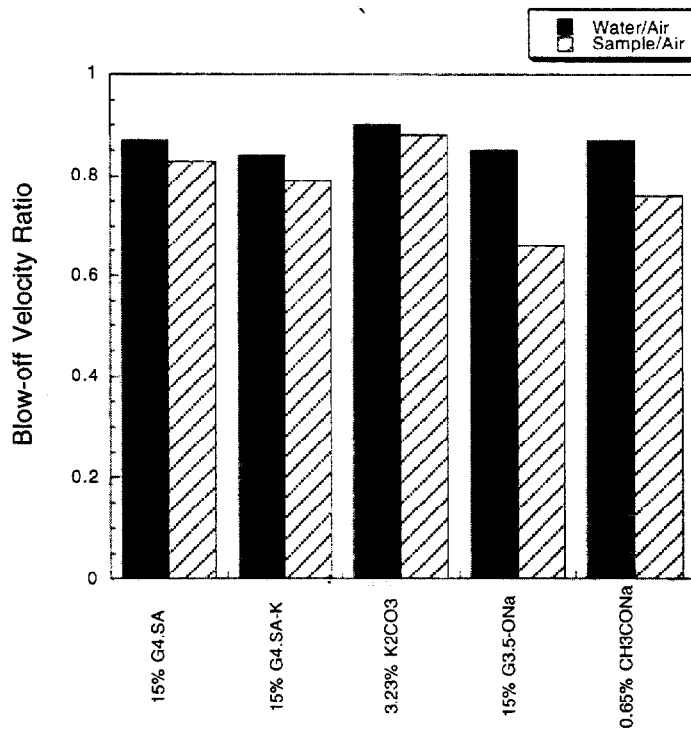
Figure 11. Blow-off Velocity Ratios for Various Candidate Agents to Air, and Reference Ratios for Water to Air Measured With the Same Conditions (pump rate of suppressant fluid to nebulizer is 0.5 ml/min in all cases).
