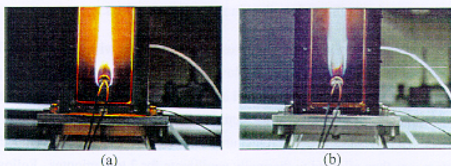
Figure 3. Picture of (a) an Envelope Flame and (b) a Wake Flame.
