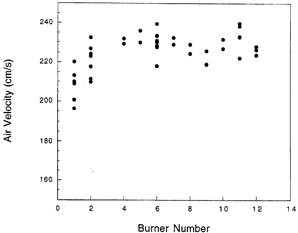
Figure 5. Air Blow-off Velocity Recorded Using Different Propane Burner Elements.
