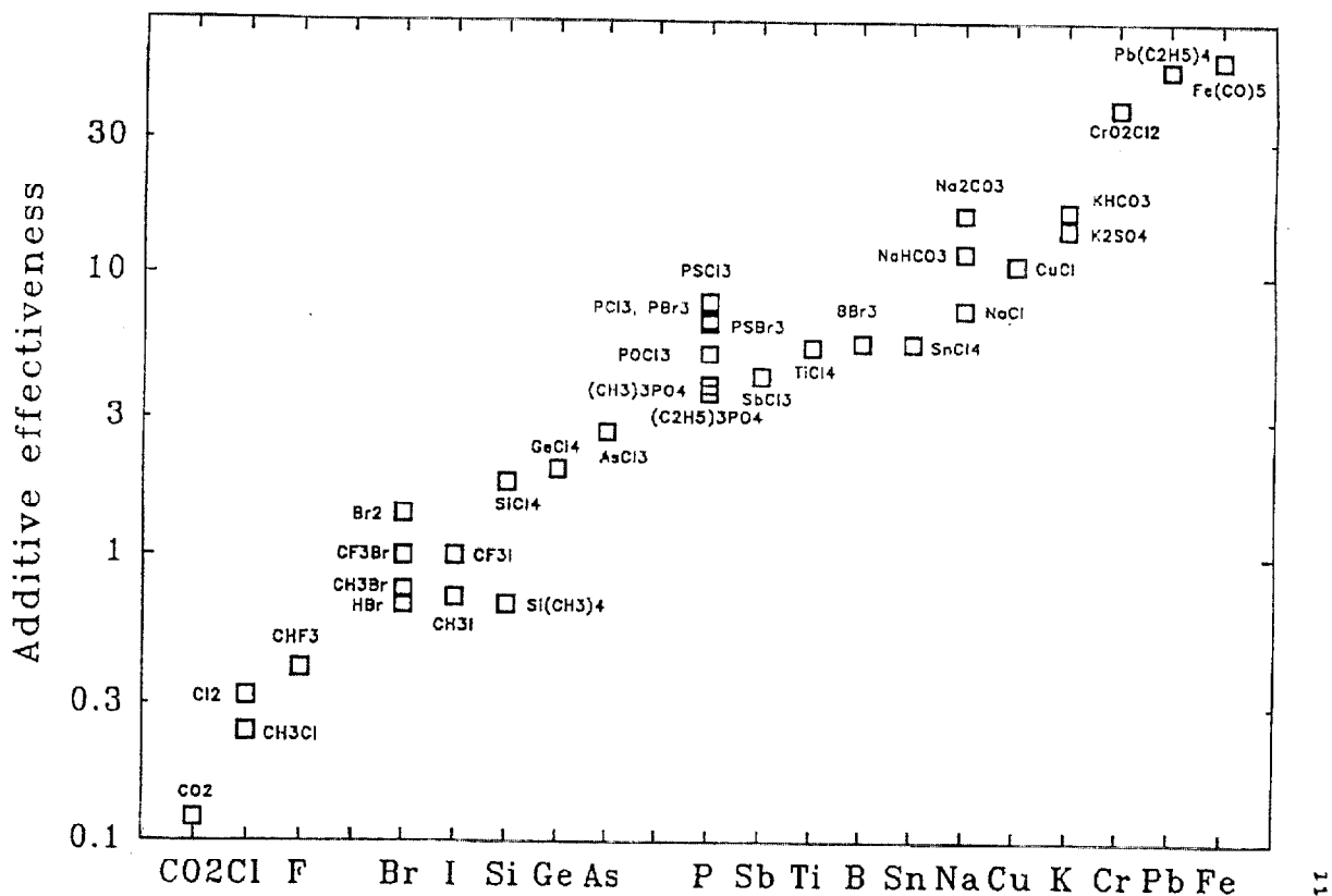
Figure 1. Chart of Fire Suppressant Effectiveness. Babushok and Tsang [4]
