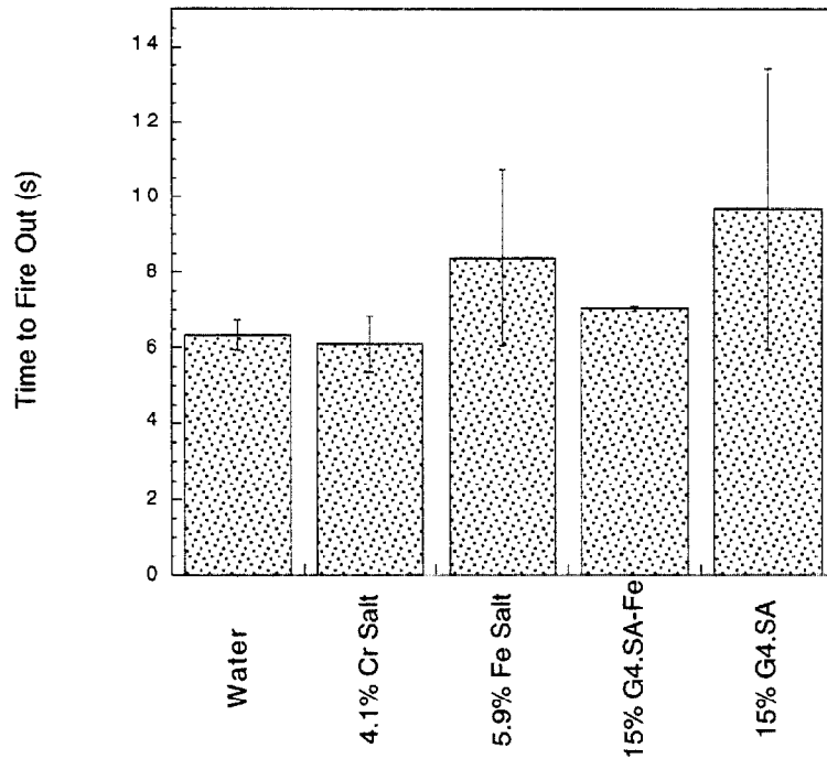
Figure 12. Times for Various Experimental Fire Suppression Agents to Extinguish a 200-ml JP8 Fuel Pan Fire (error bars represent \pm 1 standard deviation).
