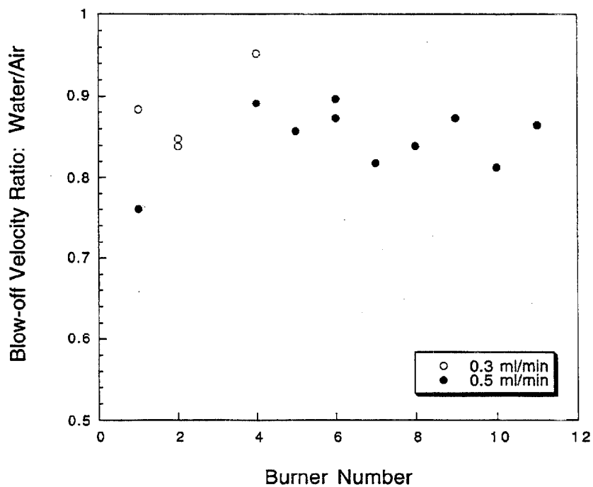
Figure 9. Ratio of Average Blow-Off Velocities Measured for Water and Air Using Different Propane Burners (open circles, water pumped to nebulizer at 0.3 ml/min; closed circles, water pumped to nebulizer at 0.5 ml/min).
