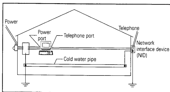
FIGURE 1.18: Power and telephone services enter the house at opposite ends. A personal computer is connected across the two systems.
