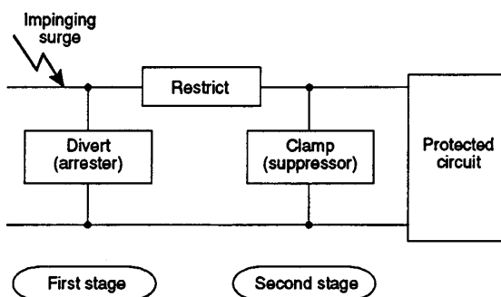
Figure 1 Two-stage surge-protection scheme
