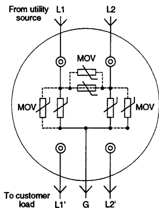
Figure 3 Internal connections of MOVs in the meter-base arresters
