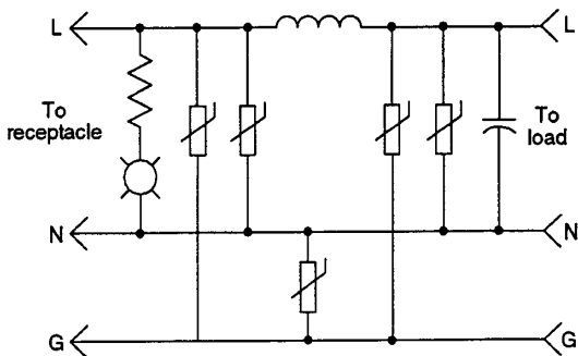
Figure 4 Typical circuit of a power-port, plug-in TVSS
