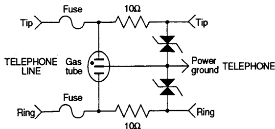
Figure 5 Typical circuit for a telephone port SRE
