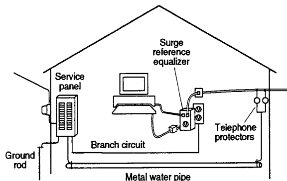
Figure 6 Surge Reference Equalizer for telephone link
